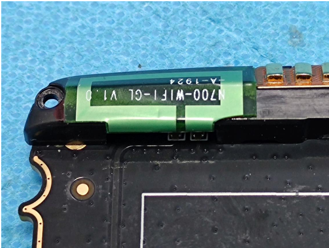
WiFi/Bluetooth Antenna
