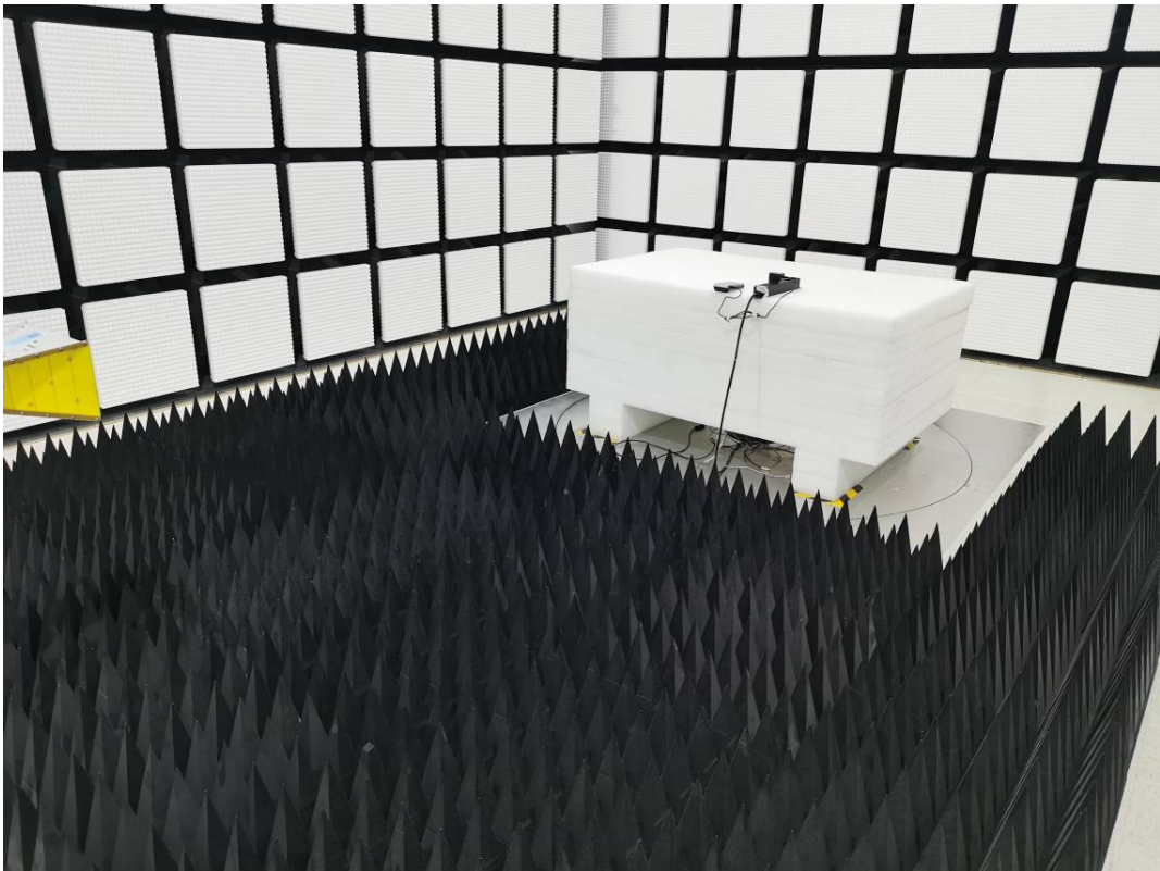
Radiated Emission Above 1G rear View
