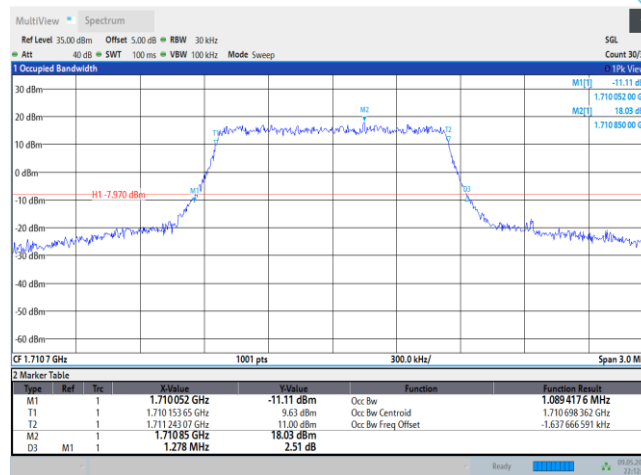
Band66-1.4MHz-QPSK-132322-6RB#0
