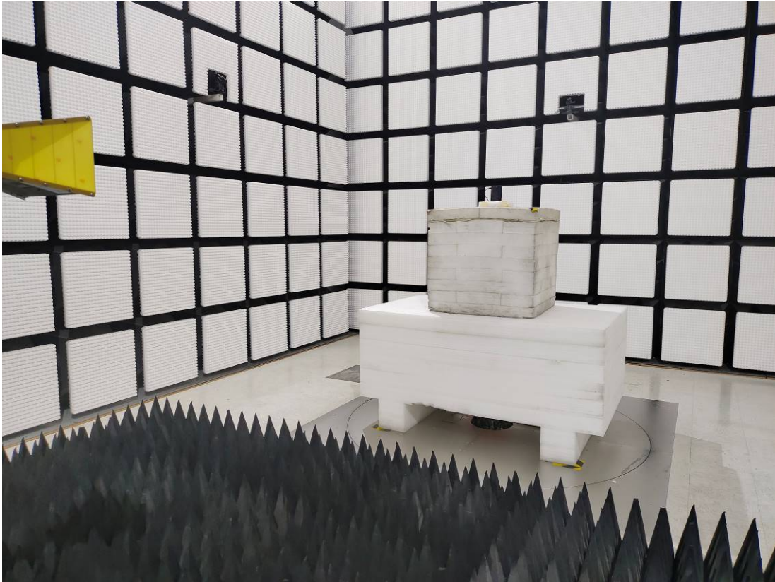
Radiated Emission Above 1GHz View-M3
