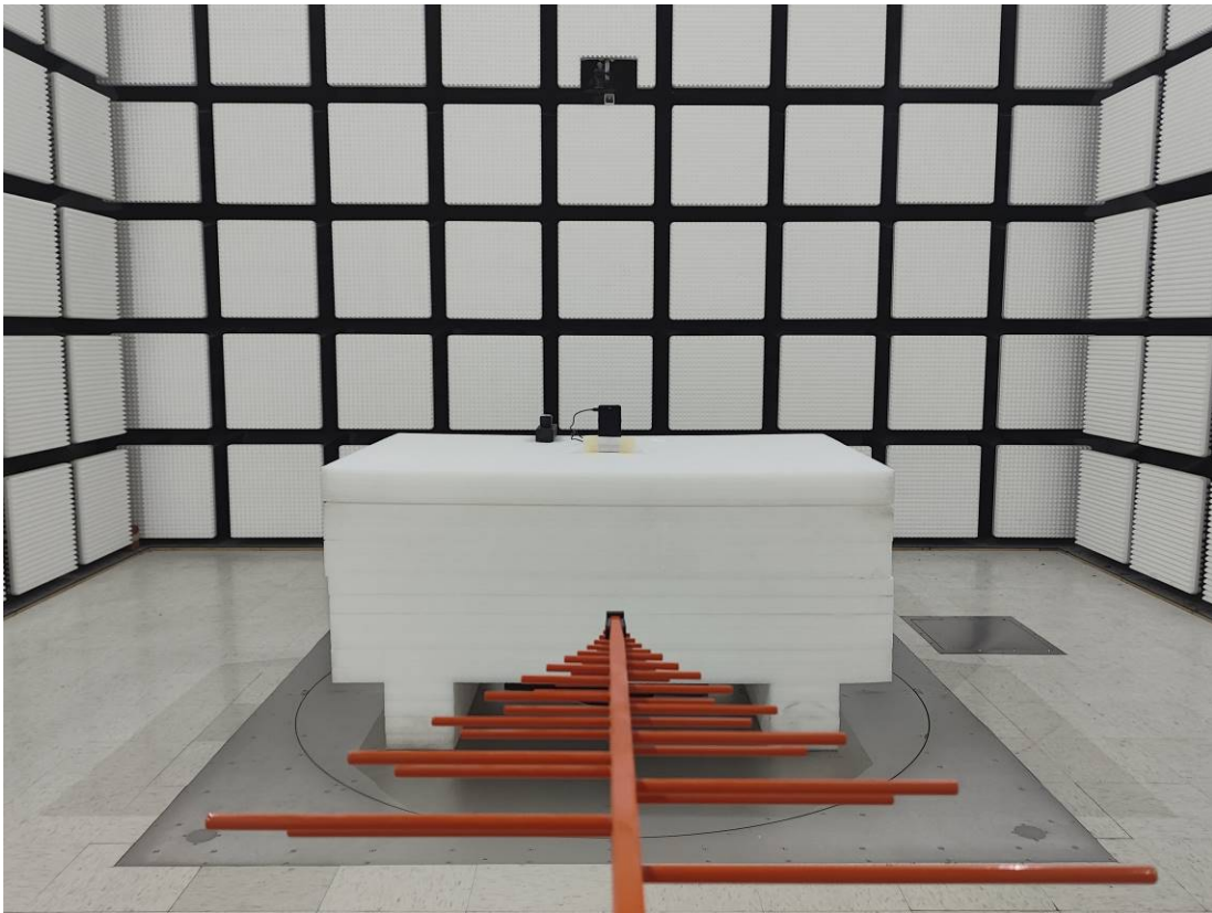
Radiated Emission Below 1GHz View-M3
