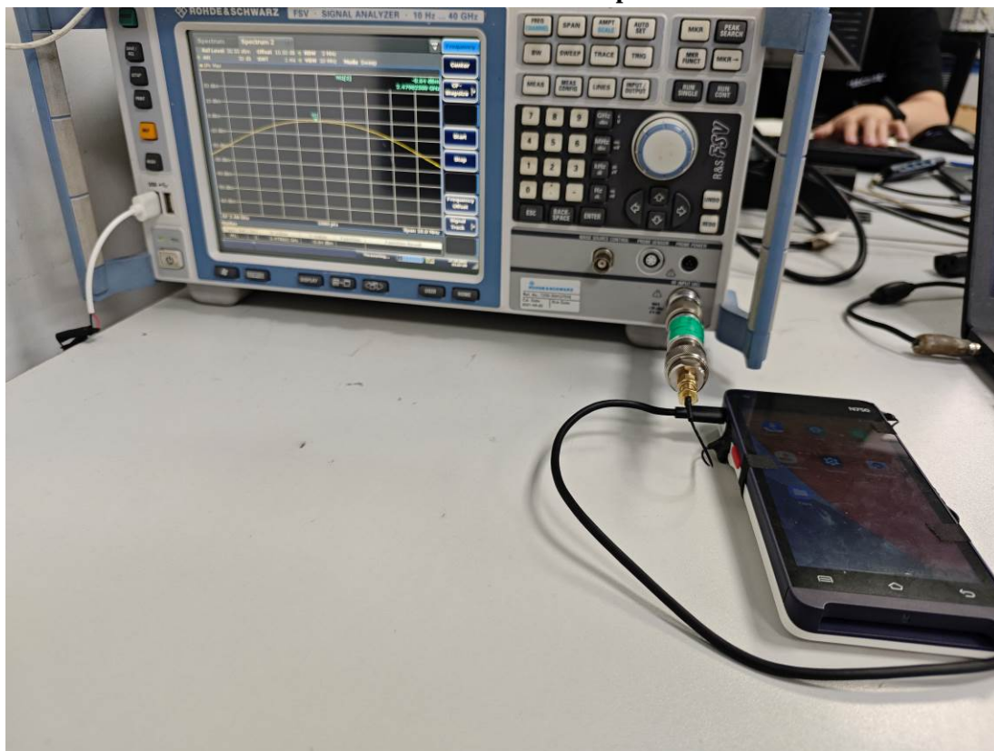
RF Conducted Test Photo for except Power item
