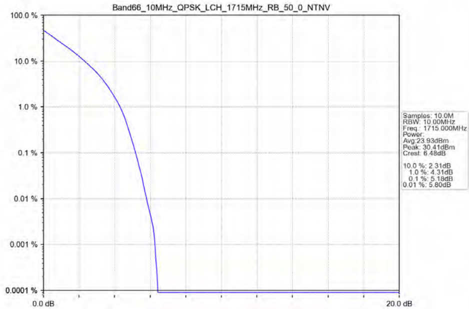
Band66_10MHz_QPSK_LCH_1715MHz_RB_50_0_NTNV
