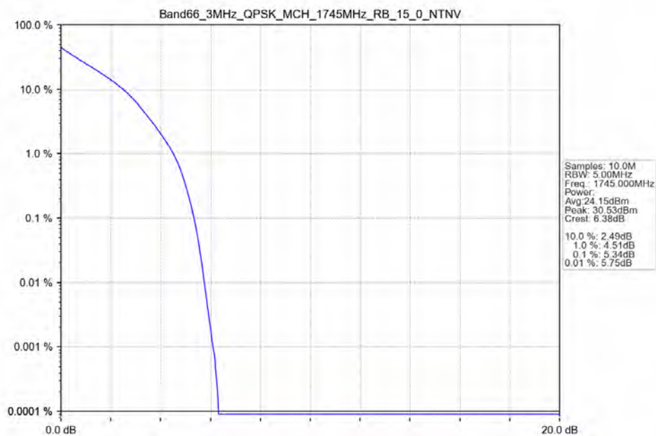
Band66_3MHz_QPSK_MCH_1745MHz_RB_15_0_NTNV
