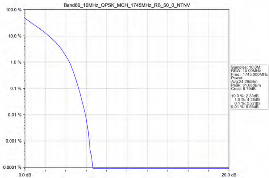
Band66_10MHz_QPSK_MCH_1745MHz_RB_50_0_NTNV
