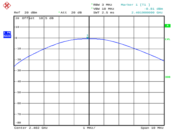
BLE_1M_Low_Channel
