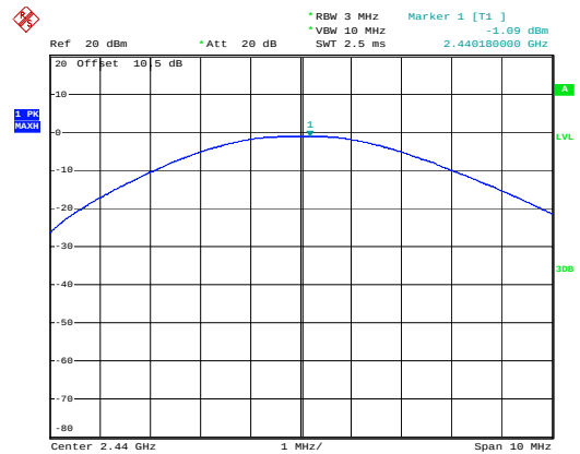
BLE_1M_Middle_Channel
