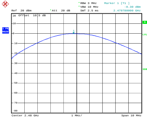
BLE_1M_High_Channel
