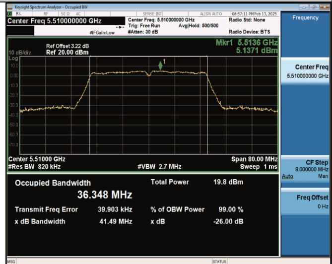
11ac40SISO-Ant0-5510
