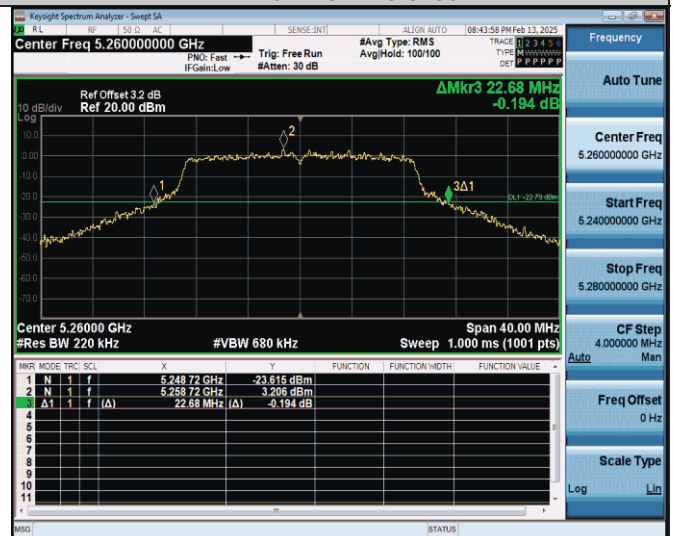
11ac20SISO-Ant0-5260
