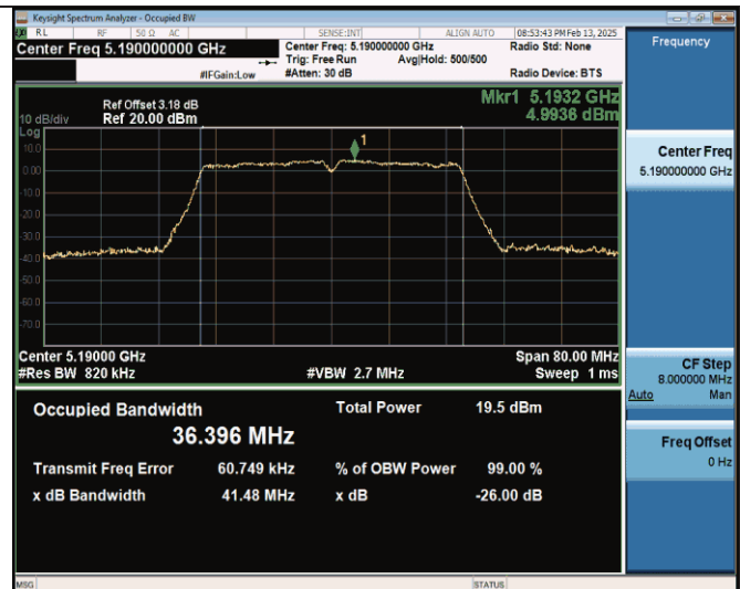
11ac40SISO-Ant0-5190
