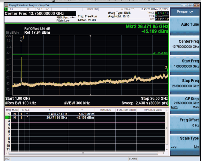
11g-Ant0-2412-1000-26500-PASS
