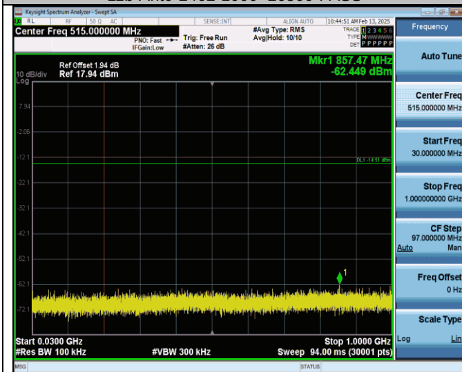
11g-Ant0-2412-30-1000-PASS
