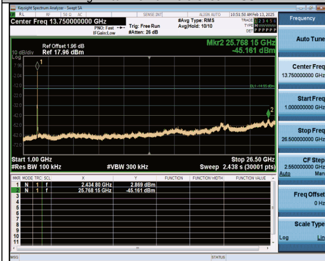
11g-Ant0-2437-1000-26500-PASS
