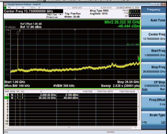
11g-Ant0-2462-1000-26500-PASS
