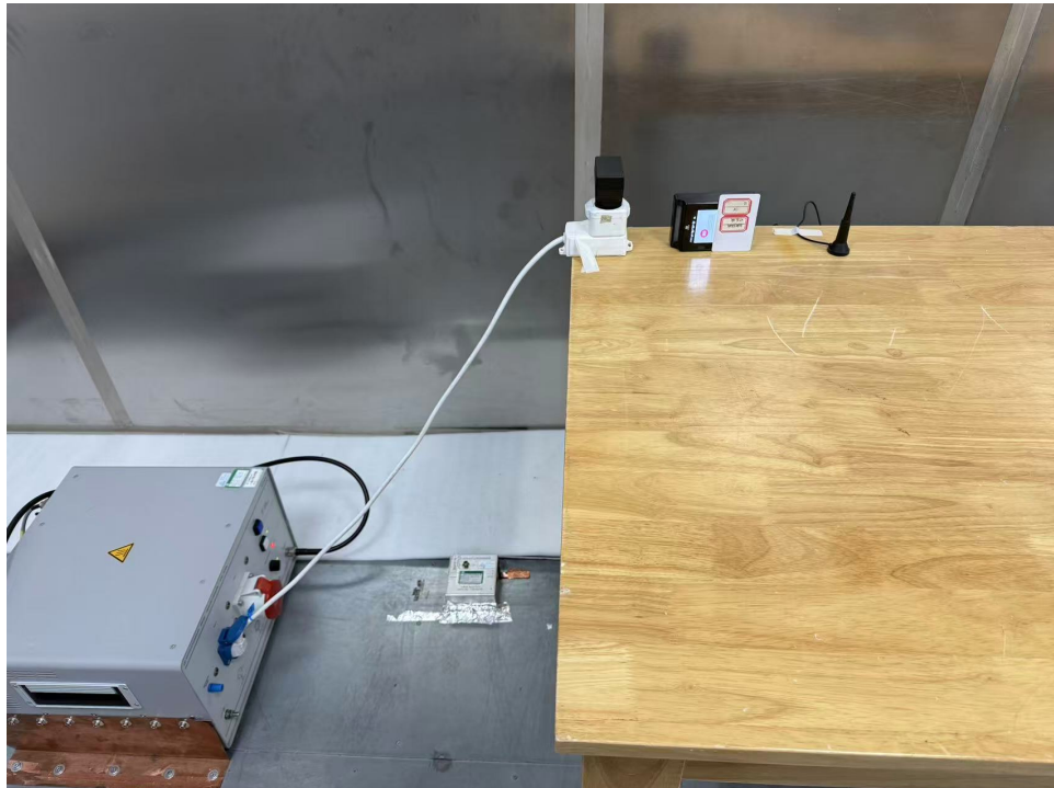
Photograph 3: Set-up photo for AC Conducted Emissions
