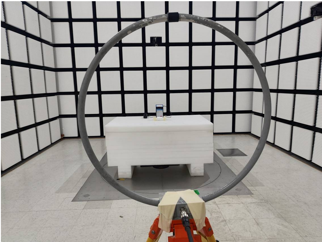
Radiated Emission Perpendicular View
