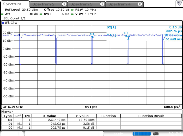
ac40_5190MHz_Chain 0
