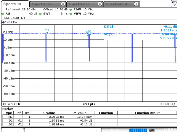
n20_5200MHz_Chain 0
