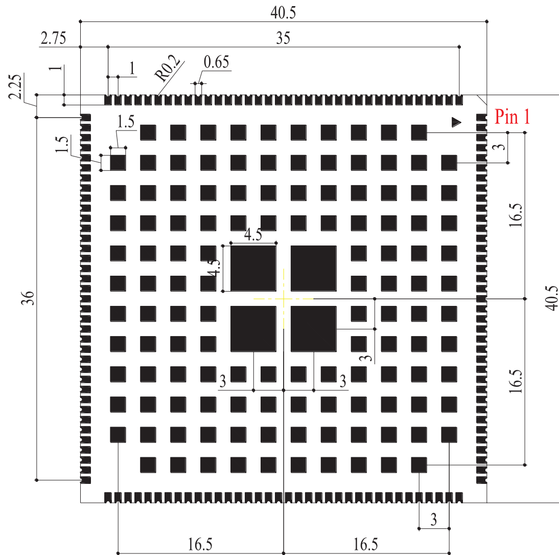
Figure 41: Module Bottom Dimensions (Bottom View)
