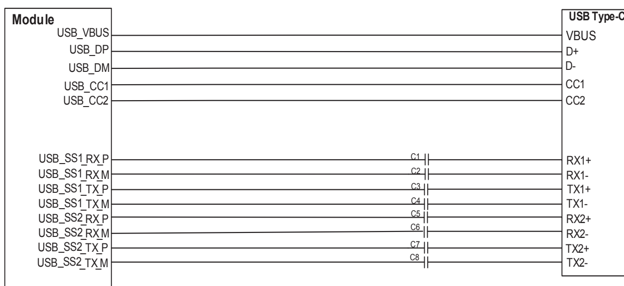
Figure 12: USB Interface Reference Design (OTG Supported)
