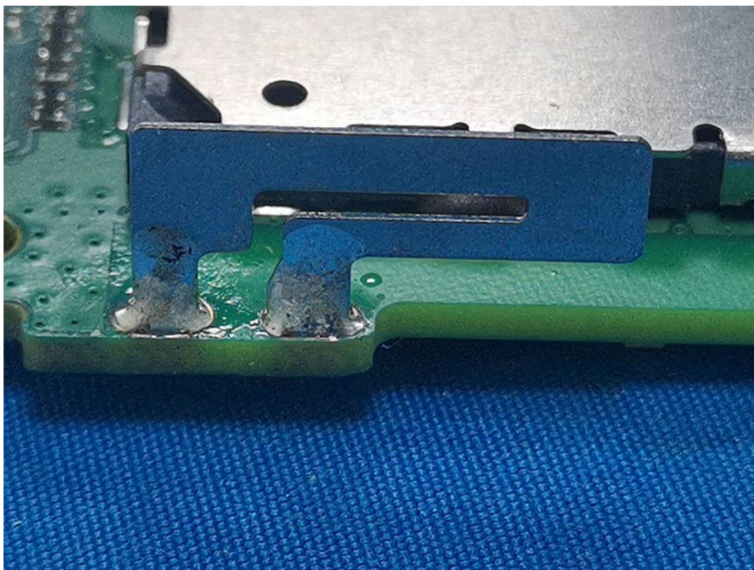
WLAN Antenna
