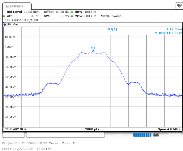
BLE_1M_Low_Channel
