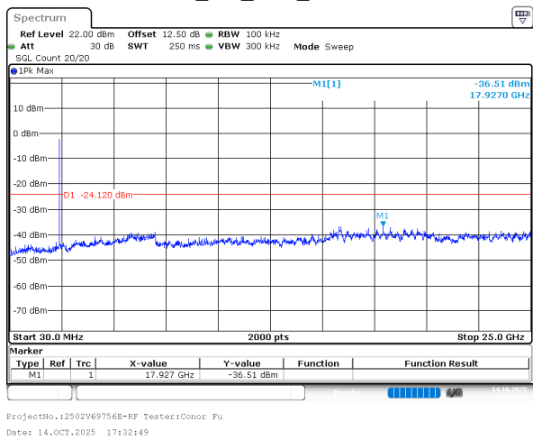
BLE_1M_Middle_Channel
