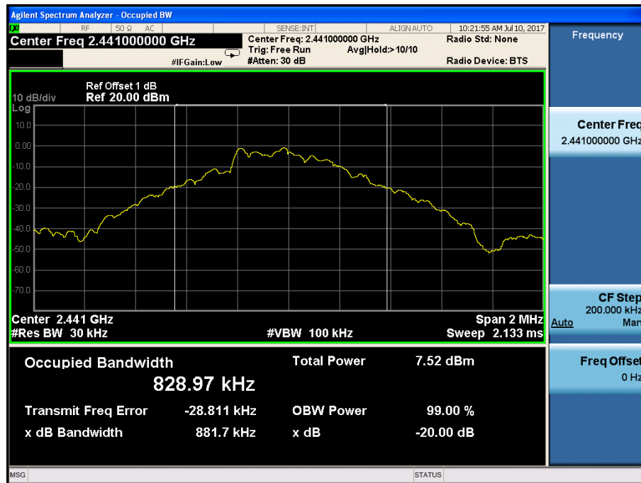
(Plot 4.4.1 B: Channel 39: 2441MHz @ GFSK)
