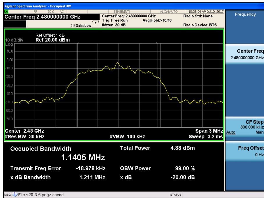
(Plot 4.4.2 C: Channel 78: 2480MHz @ 8DPSK)
