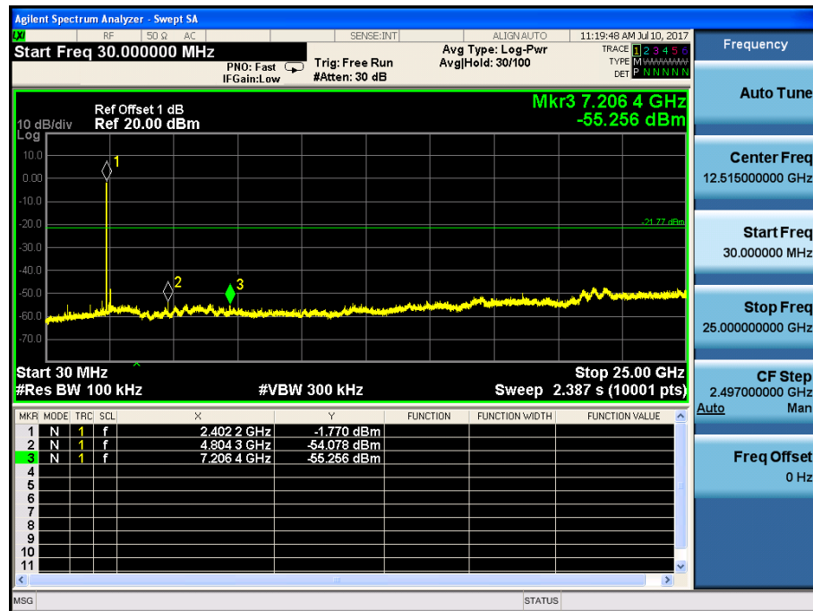
(Plot 4.9.1 A: Channel 00: 2402MHz @ GFSK)
