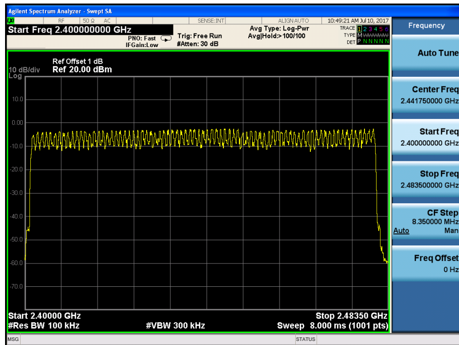
(Plot 4.7.2 A1: @ 8DPSK)
