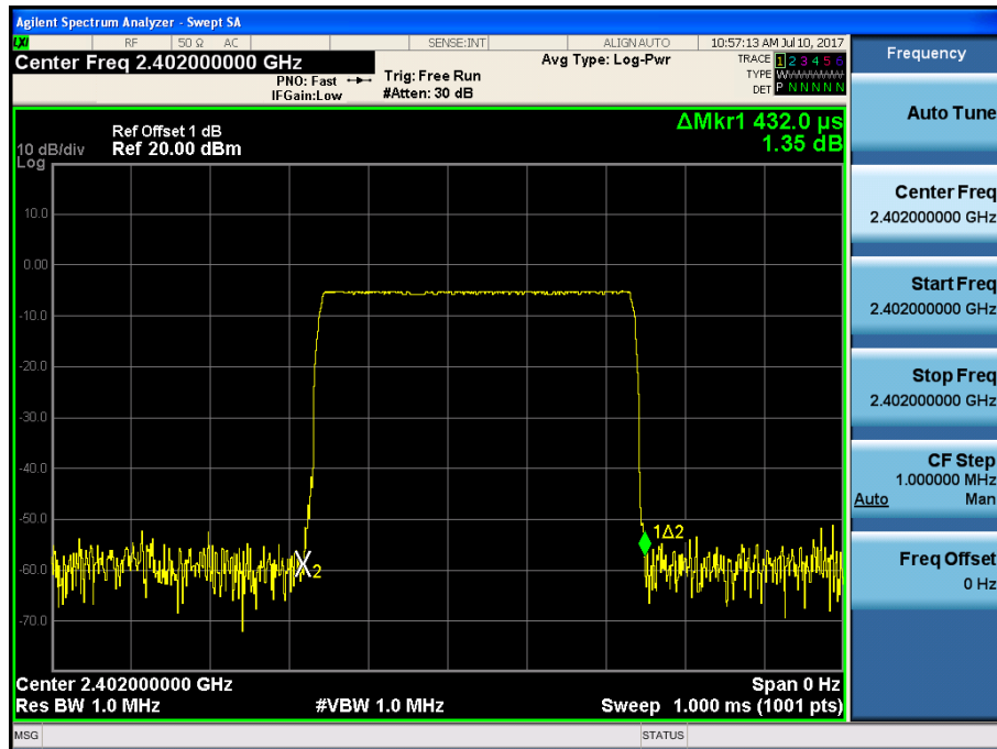
(Plot 4.8.1.A: Channel 00: 2402MHz @ GFSK @ DH1)
