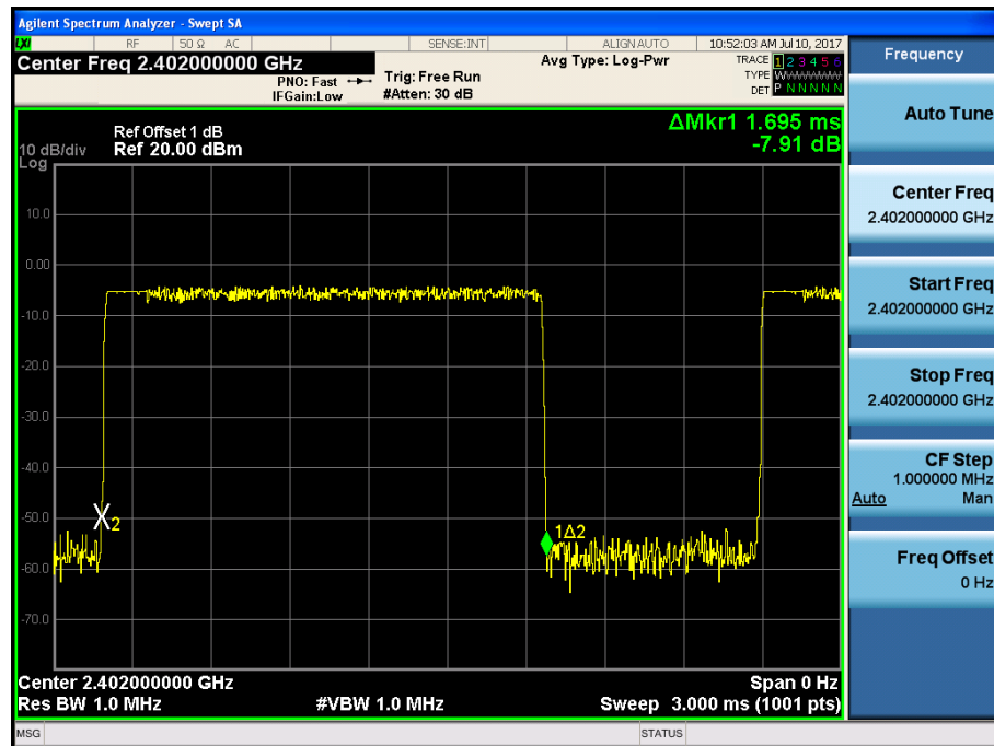
(Plot 4.8.2.B: Channel 00: 2402MHz @ 8DPSK @ DH3)
