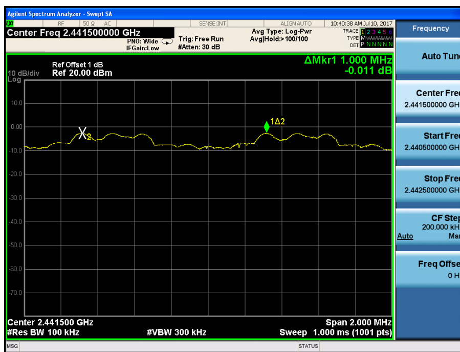
(Plot 4.6.2 A: Channel 39: 2441MHz @ 8DPSK)
