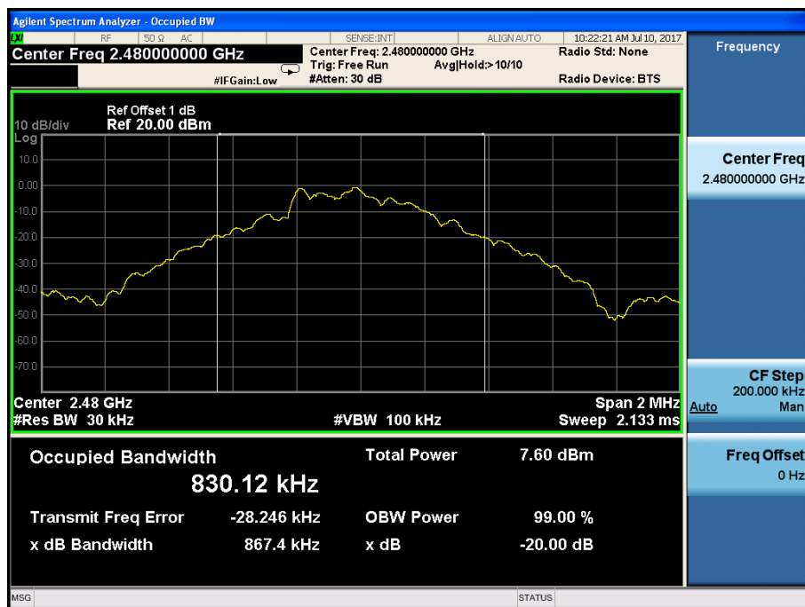
(Plot 4.4.1 C: Channel 78: 2480MHz @ GFSK)
