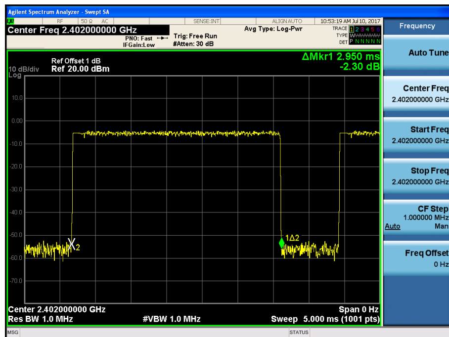
(Plot 4.8.2.C: Channel 00: 2402MHz @ 8DPSK @ DH5)
