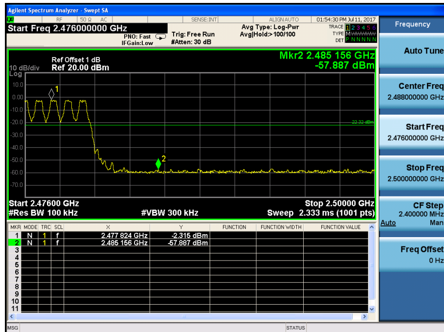
(Plot 4.5.2.1 B: Hopping Mode @ GFSK)
