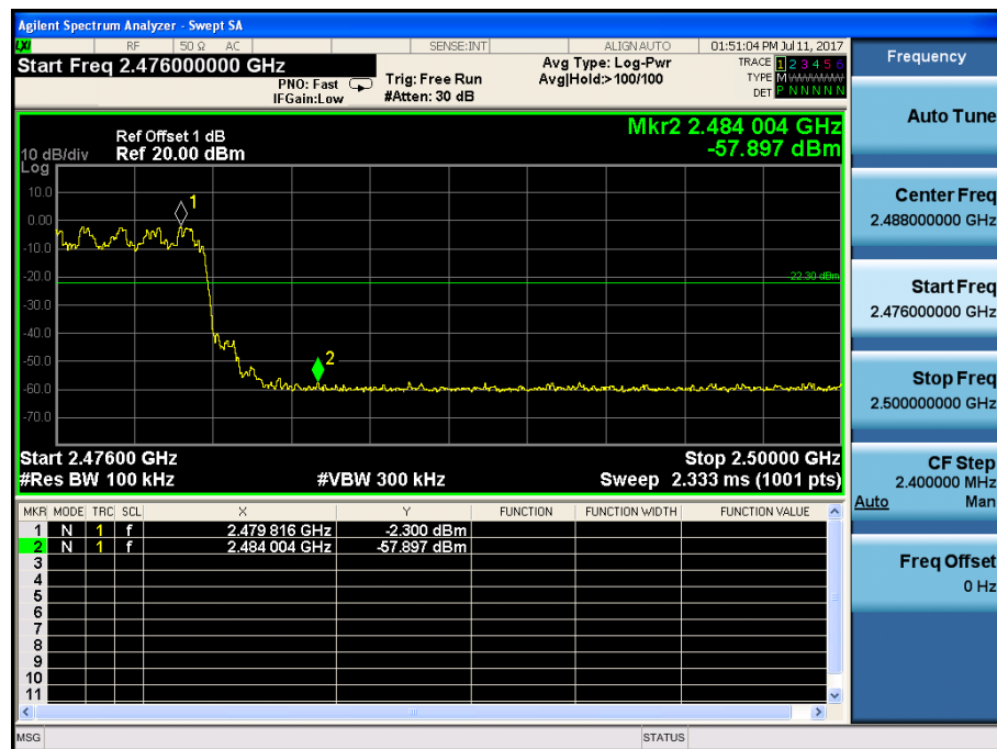
(Plot 4.5.2.2 B: Hopping Mode @ 8DPSK)
