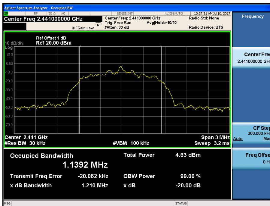
(Plot 4.4.2 B: Channel 39: 2441MHz @ 8DPSK)
