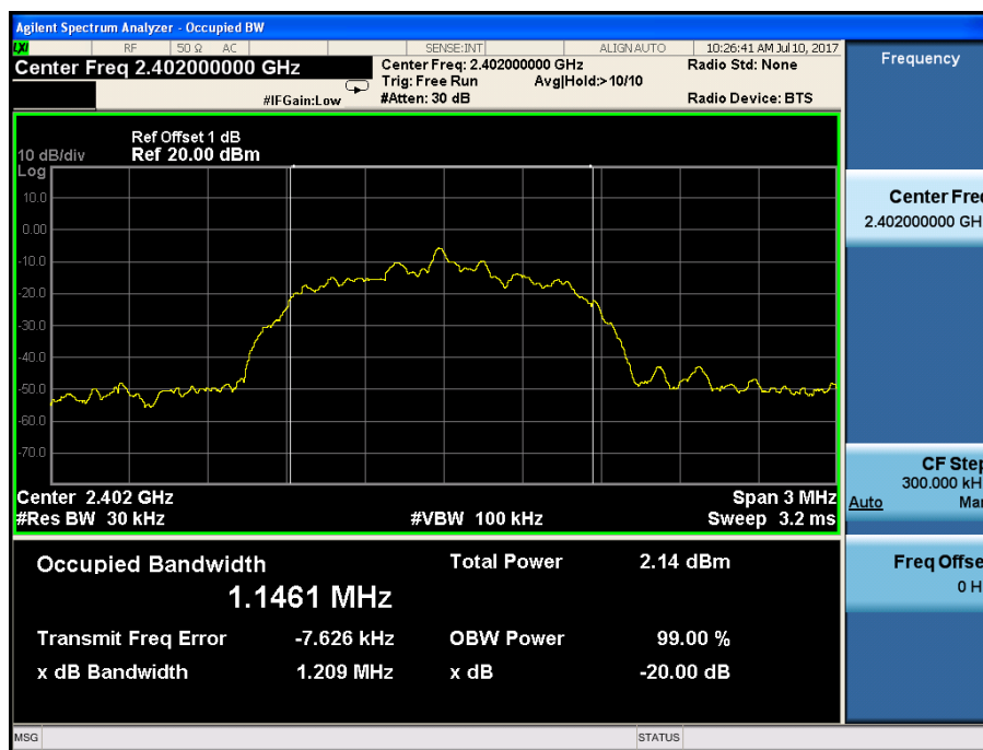
(Plot 4.4.2 A: Channel 00: 2402MHz @ 8DPSK)
