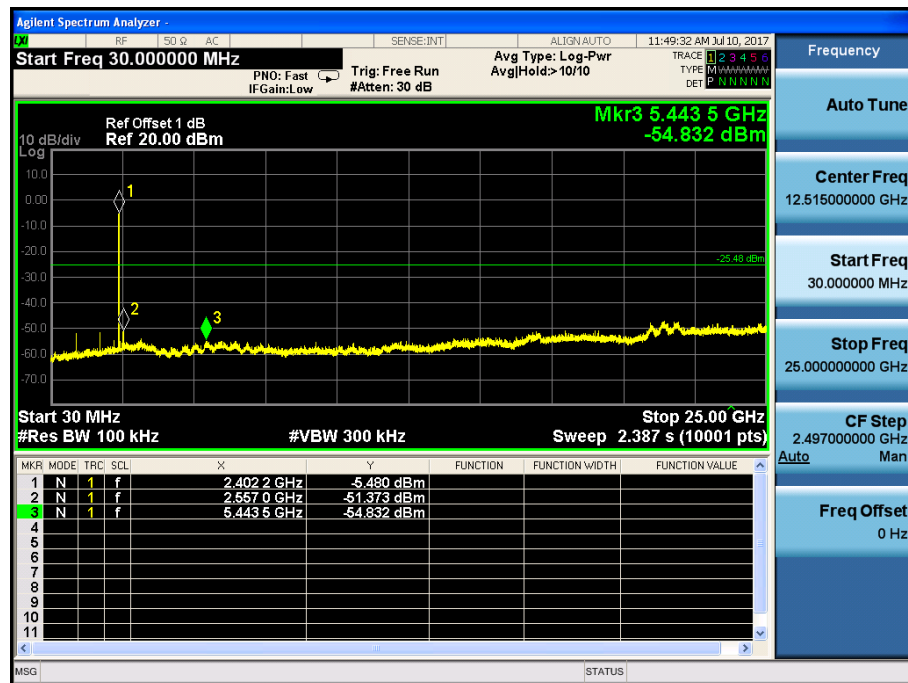
(Plot 4.9.2 A: Channel 00: 2402MHz @ 8DPSK)
