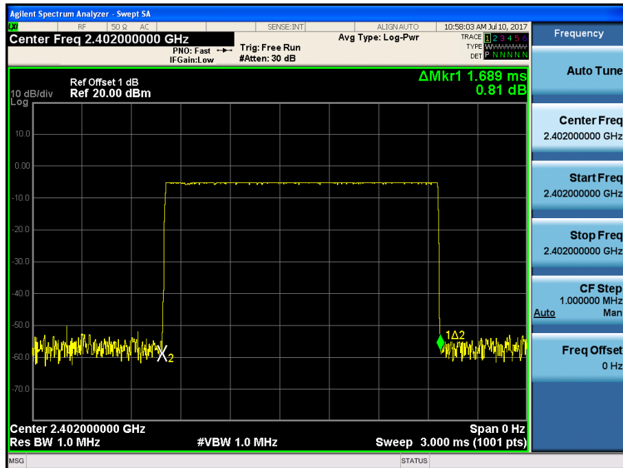
(Plot 4.8.1.B: Channel 00: 2402MHz @ GFSK @ DH3)
