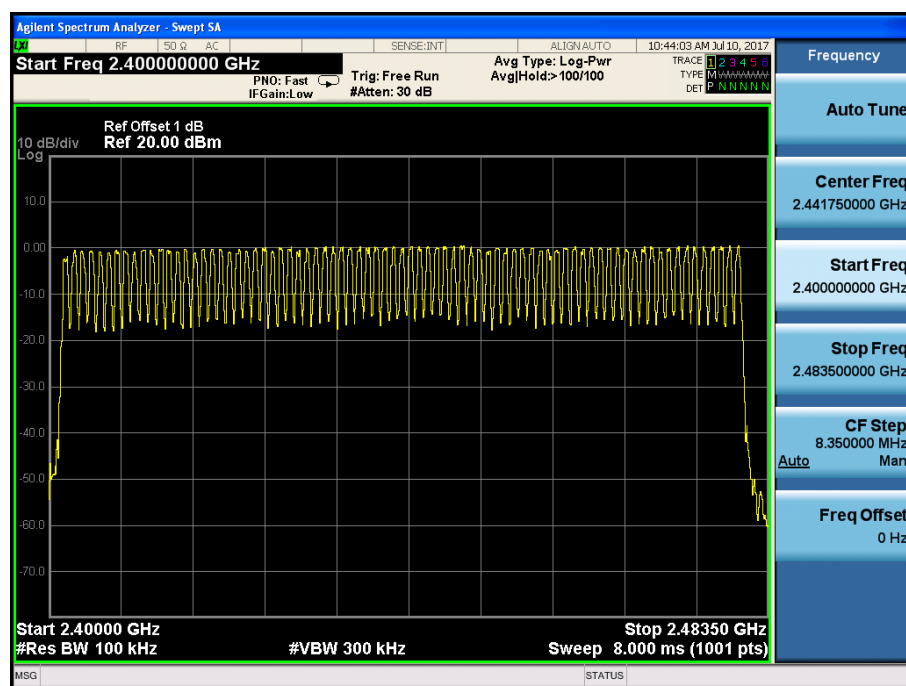
(Plot 4.7.1 A1: @ GFSK)
