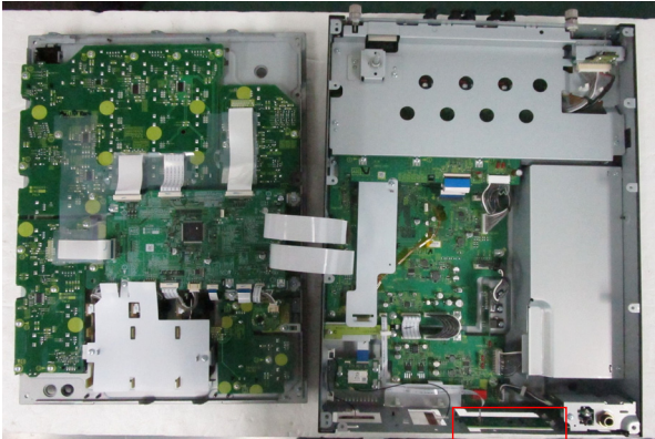
[Wireless Module Area (Front)]
