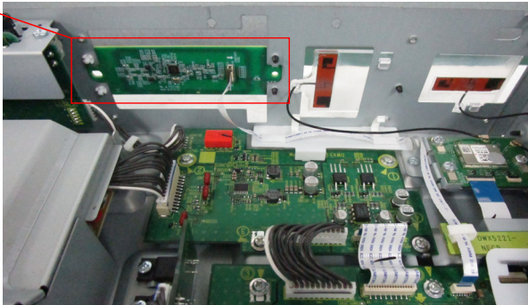
[Wireless Module Area (Rear)]
