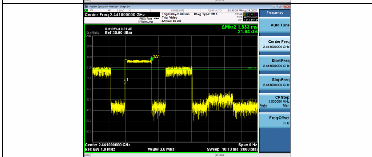
2DH3-Ant1-Hop-PASS
