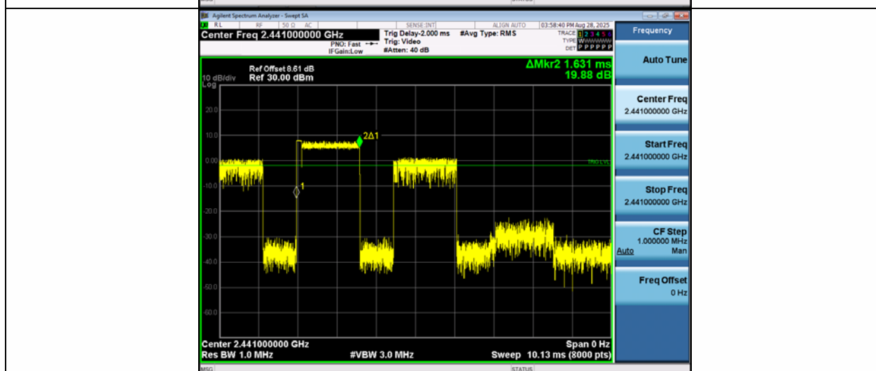
3DH3-Ant1-Hop-PASS
