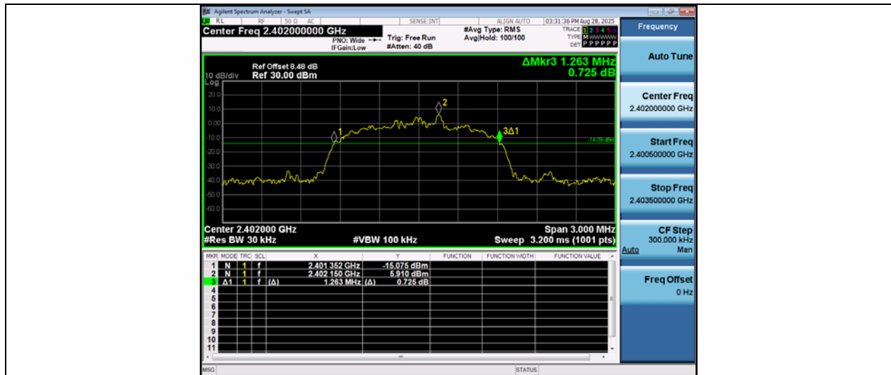
3DH5-Ant1-2402
