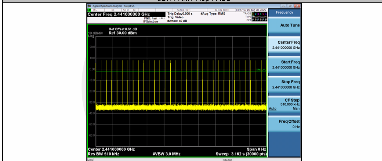
3DH1-Ant1-Hop-PASS
