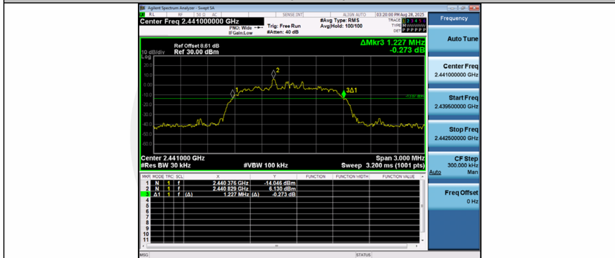
2DH5-Ant1-2441
