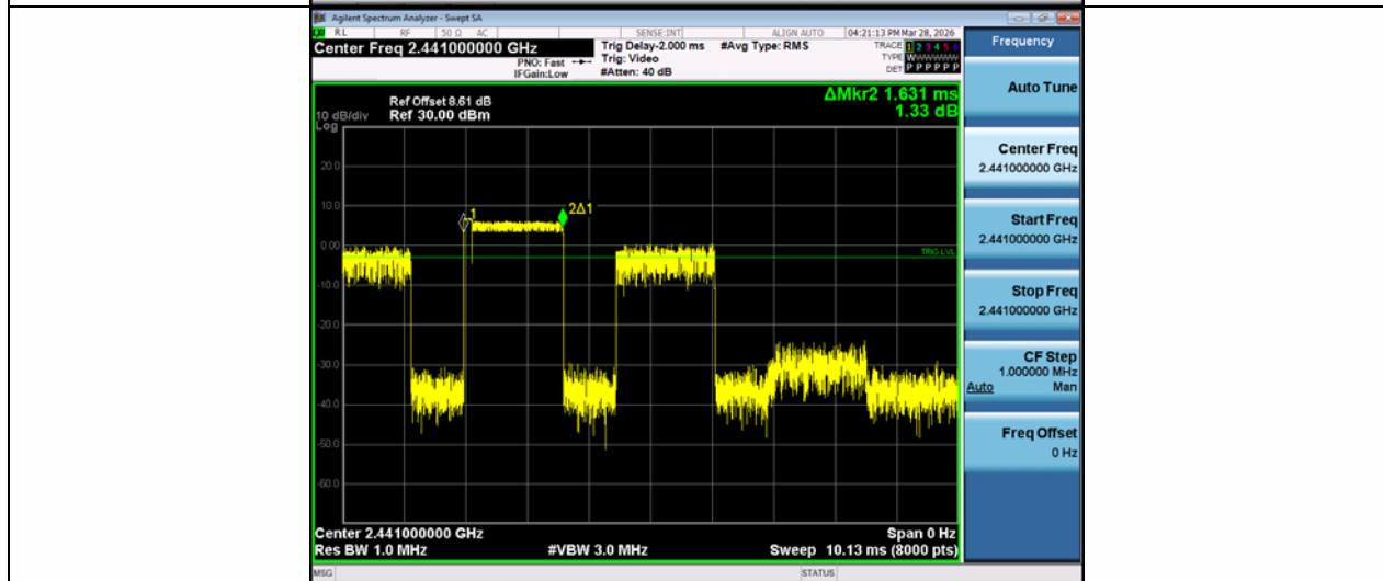
2DH3-Ant1-Hop-PASS
