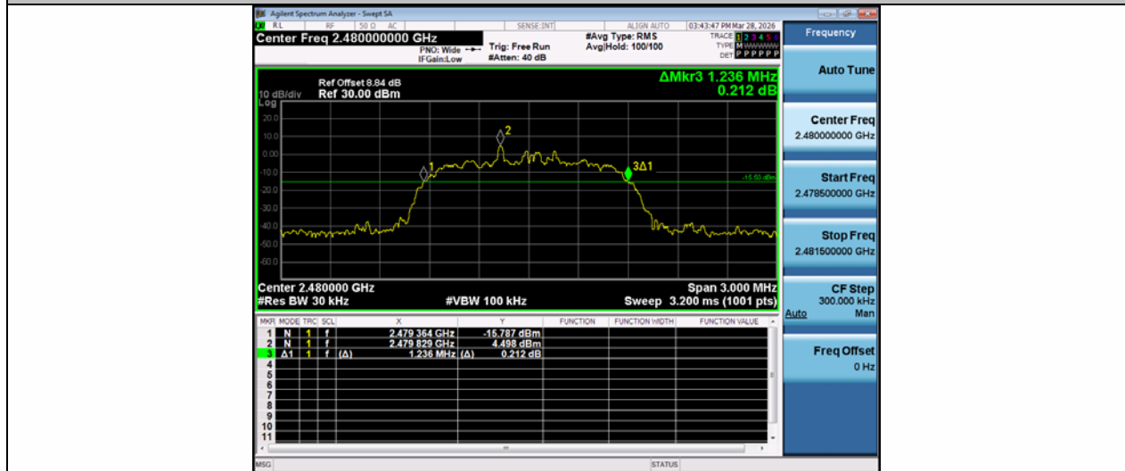
2DH5-Ant1-2480
