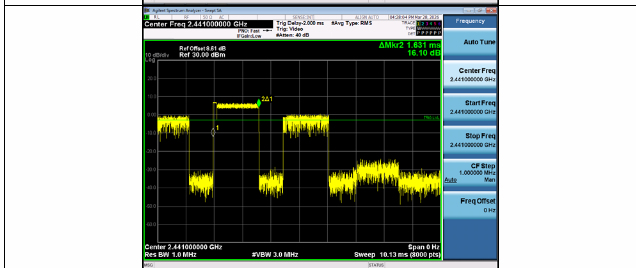
3DH3-Ant1-Hop-PASS
