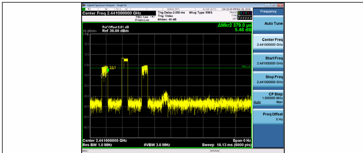
3DH1-Ant1-Hop-PASS
