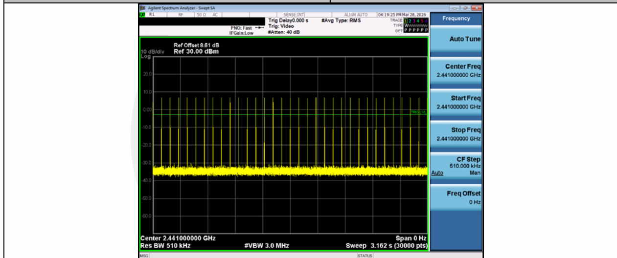
2DH1-Ant1-Hop-PASS
