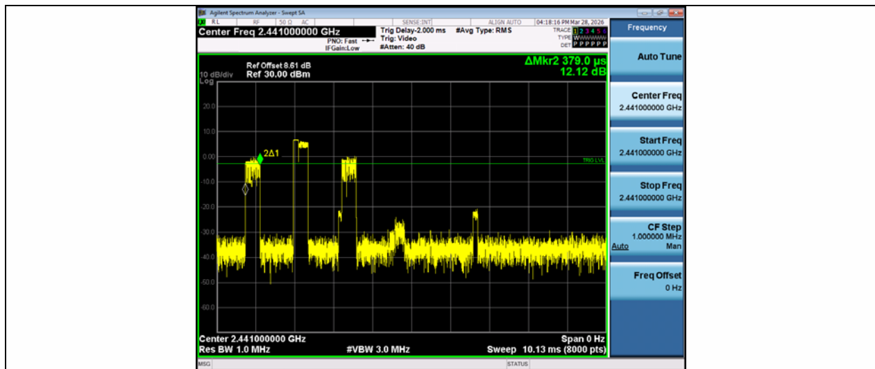
2DH1-Ant1-Hop-PASS
