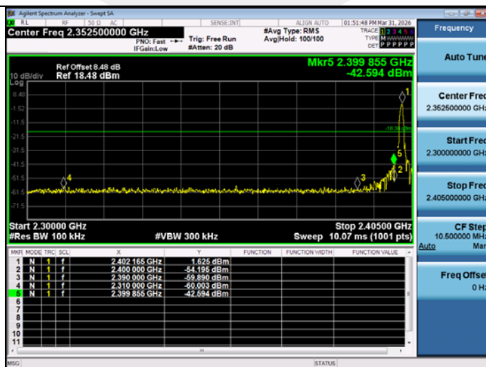
SRD-Ant2-2402-PASS
