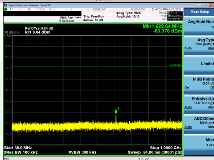
SRD-Ant1-2480-30~1000-PASS
