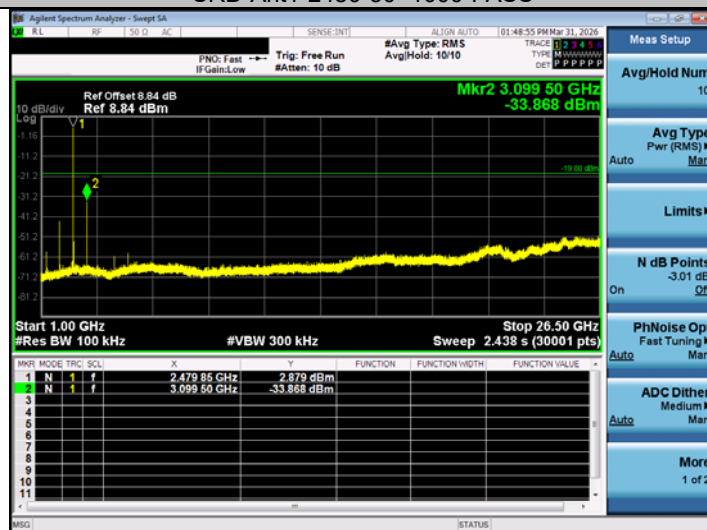
SRD-Ant1-2480-1000~26500-PASS
