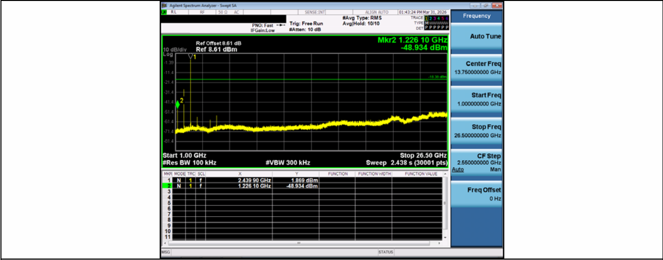
SRD-Ant1-2440-1000~26500-PASS
