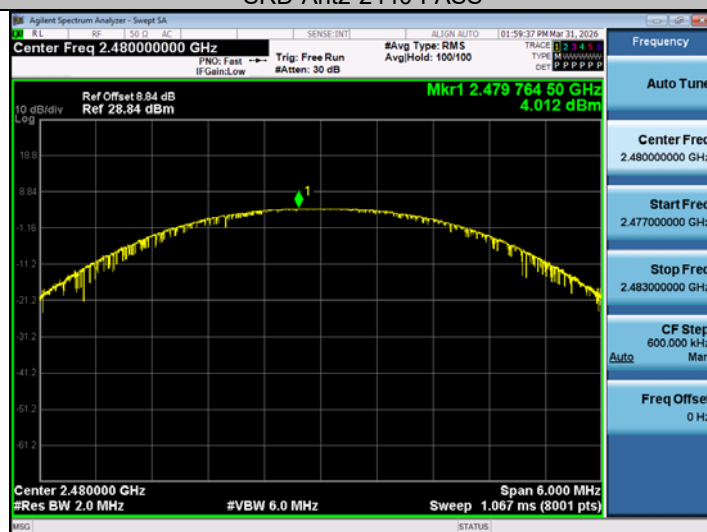
SRD-Ant2-2480-PASS
