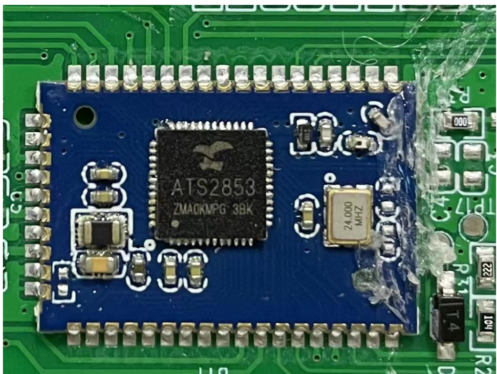
Internal Photos M/N: DM-40D-BT-W
