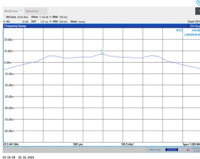
SRD2.4G_Ant1_2441
