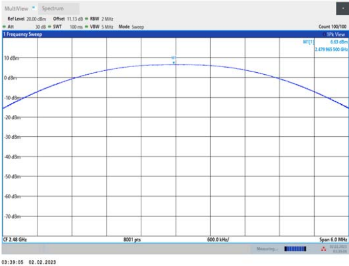
SRD2.4G_Ant2_2480
