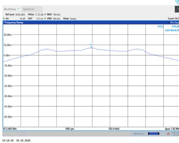
SRD2.4G_Ant2_2402
