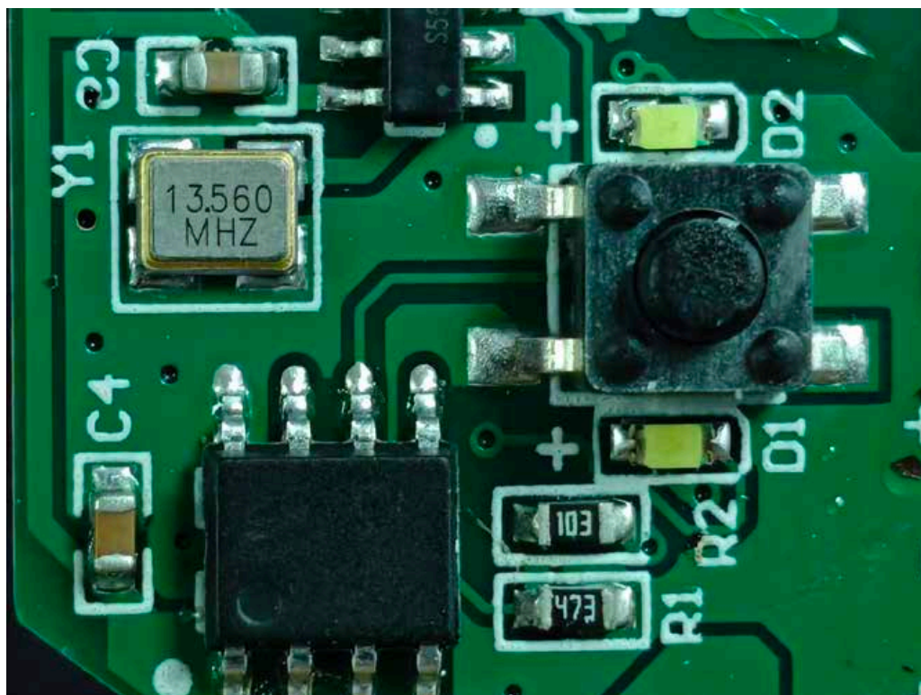
FIGURE 10 USB RECHARGEABLE REMOTE CONTROL (RE-003) CRYSTAL ON MAINBOARD
