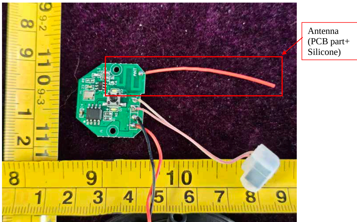
FIGURE 8 USB RECHARGEABLE REMOTE CONTROL (RE-003) MAINBOARD FRONT
