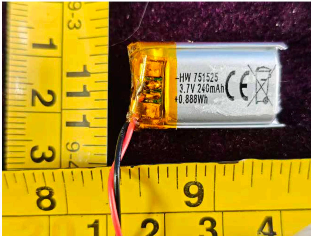
FIGURE 11 USB RECHARGEABLE REMOTE CONTROL (RE-003) BATTERY
