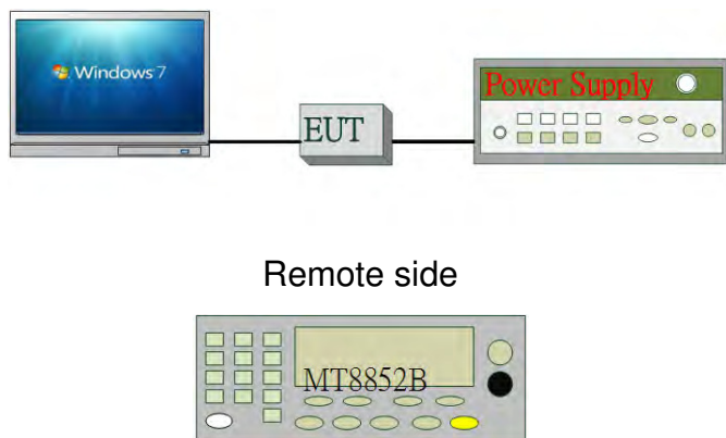
Fig. 2-1 Conducted (Antenna Port) Emission Configuration
