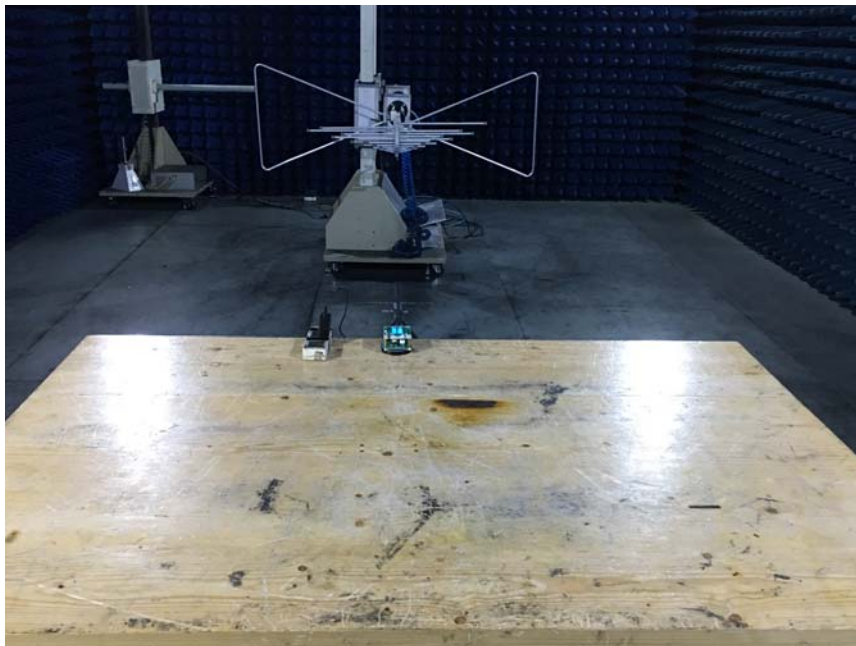
Photograph of set-up for Radiated Emission From 30MHz-1GHz
