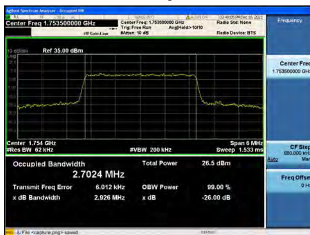
Band4 / 3MHz / High CH / 64QAM
