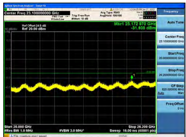
Band38-20G-26G / 20MHz / Mid CH / QPSK
