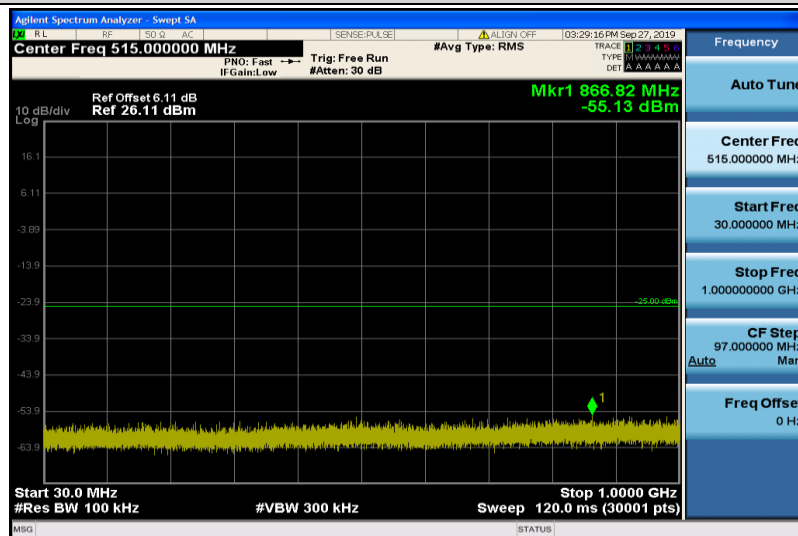
Band7-5MHz-QPSK-21100-1RB#0-30~1000MHz
