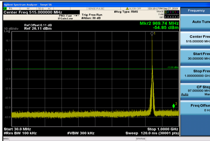
Band5-5MHz-QPSK-20625-1RB#0-30~1000MHz
