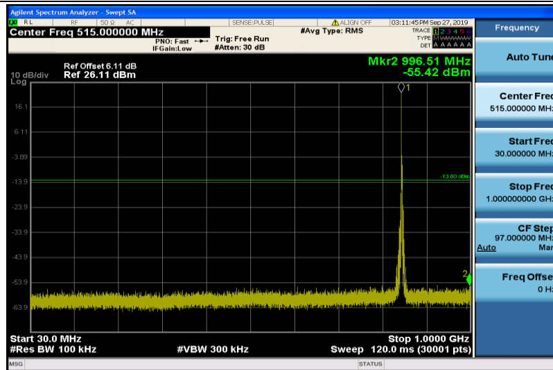
Band5-3MHz-16QAM-20635-1RB#0-30~1000MHz
