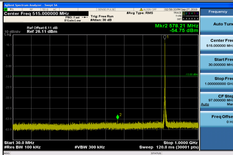
Band5-1.4MHz-QPSK-20407-1RB#0-30~1000MHz
