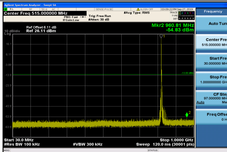
Band5-3MHz-16QAM-20415-1RB#0-30~1000MHz
