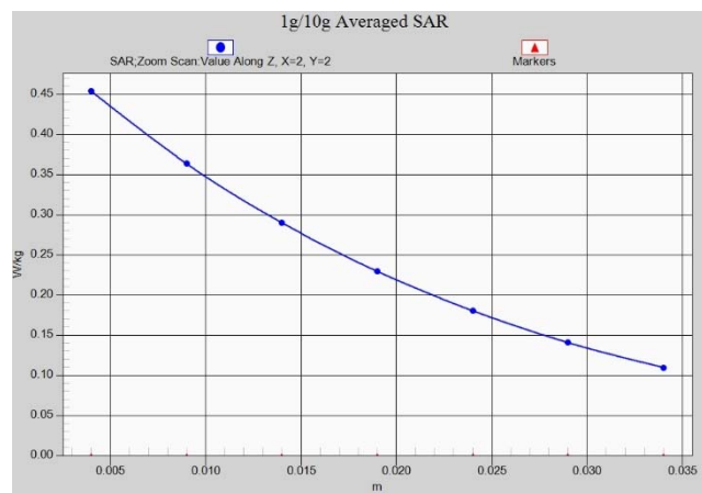
Fig.A.1- 26 Z-Scan at power reference point (LTE band13)
