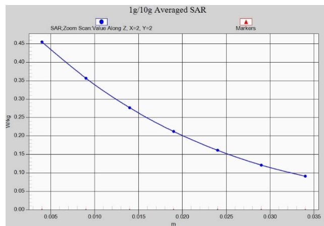
Fig.A.1- 12 Z-Scan at power reference point (CDMA BC0)
