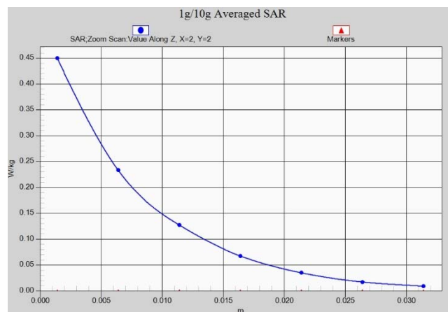
Fig.A.1- 36 Z-Scan at power reference point (LTE band41 PC2)
