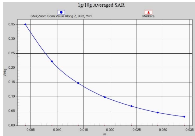
Fig.A.1- 13 Z-Scan at power reference point (CDMA BC1)
