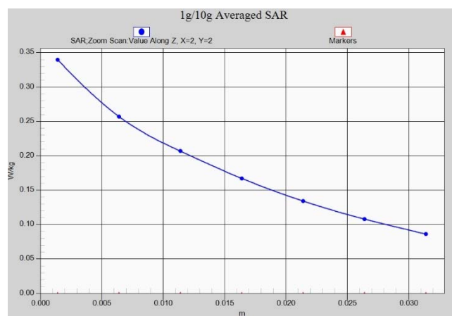
Fig.A.1- 29 Z-Scan at power reference point (LTE band26)
