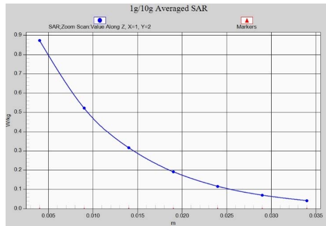
Fig.A.1- 28 Z-Scan at power reference point (LTE band25)
