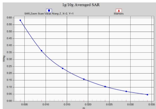
Fig.A.1- 27 Z-Scan at power reference point (LTE band25)
