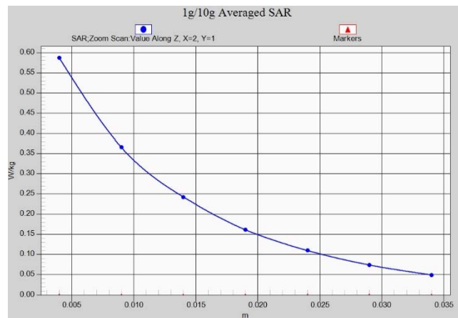
Fig.A.1- 17 Z-Scan at power reference point (LTE band2)
