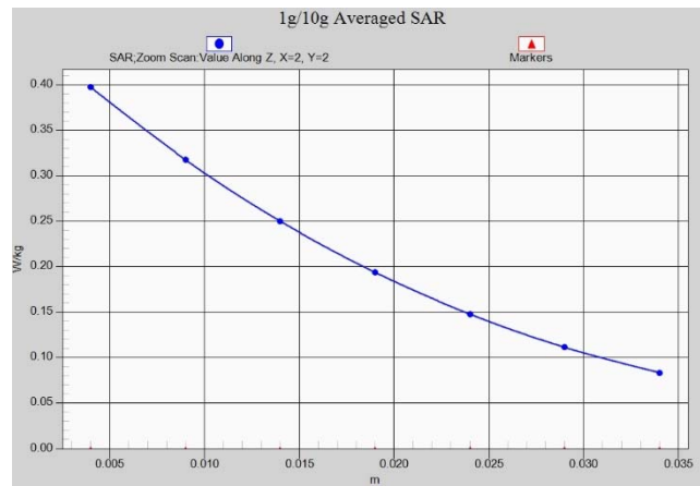
Fig.A.1- 22 Z-Scan at power reference point (LTE band5)
