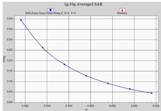
Fig.A.1- 19 Z-Scan at power reference point (LTE band4)
