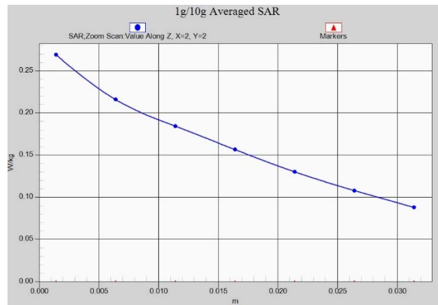
Fig.A.1- 25 Z-Scan at power reference point (LTE band13)
