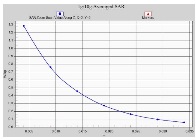
Fig.A.1- 14 Z-Scan at power reference point (CDMA BC1)
