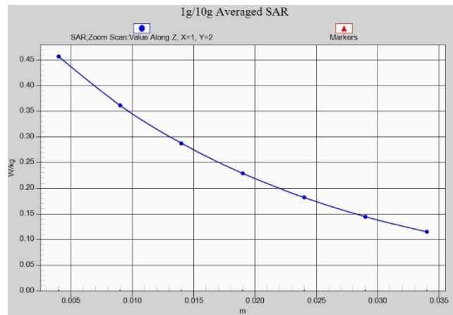
Fig.A.1- 16 Z-Scan at power reference point (CDMA BC10)
