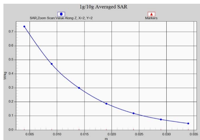
Fig.A.1- 20 Z-Scan at power reference point (LTE band4)
