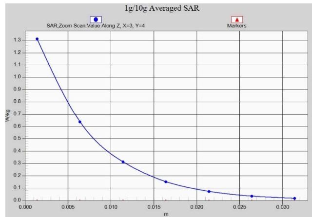
Fig.A.1- 40 Z-Scan at power reference point (Wifi2450)
