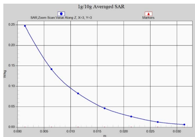
Fig.A.1- 32 Z-Scan at power reference point (LTE band41 PC3)
