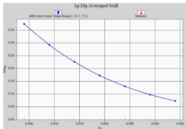
Fig.A.1- 30 Z-Scan at power reference point (LTE band26)
