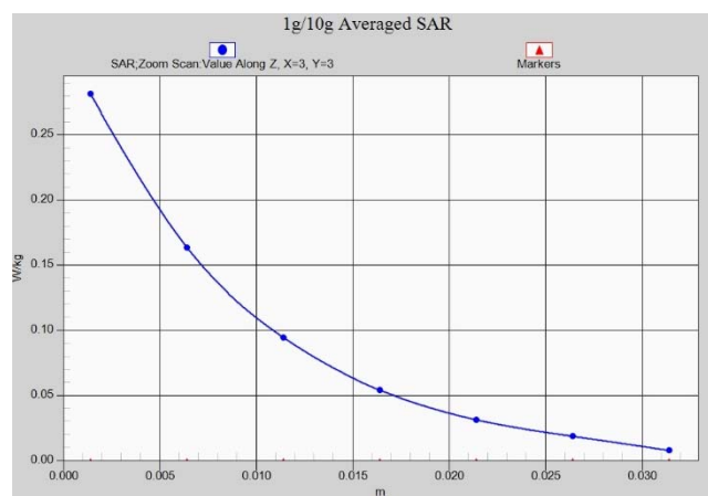
Fig.A.1- 35 Z-Scan at power reference point (LTE band41 PC2)
