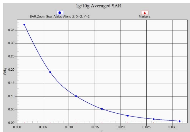
Fig.A.1- 33 Z-Scan at power reference point (LTE band41 PC3)
