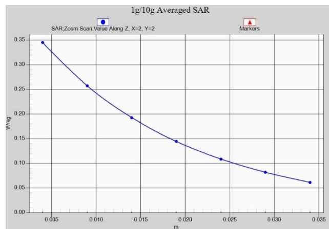
Fig.A.1- 24 Z-Scan at power reference point (LTE band12)
