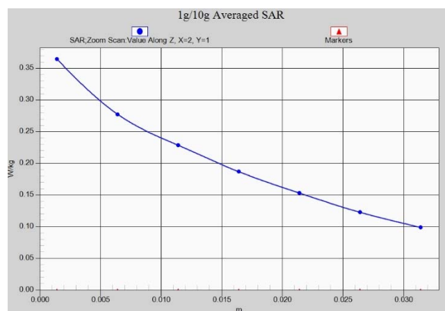
Fig.A.1- 15 Z-Scan at power reference point (CDMA BC10)
