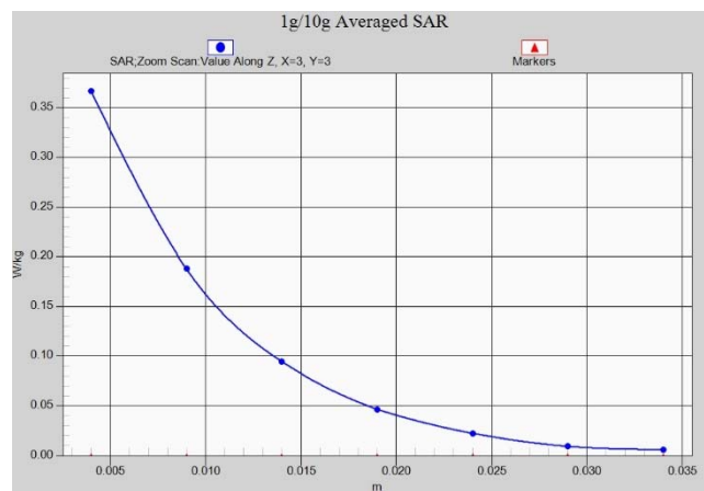
Fig.A.1- 39 Z-Scan at power reference point (Wifi2450)
