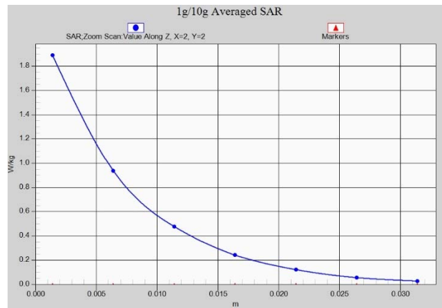
Fig.A.1- 34 Z-Scan at power reference point (LTE band41 PC2)
