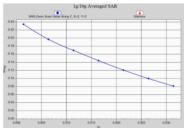
Fig.A.1- 23 Z-Scan at power reference point (LTE band12)
