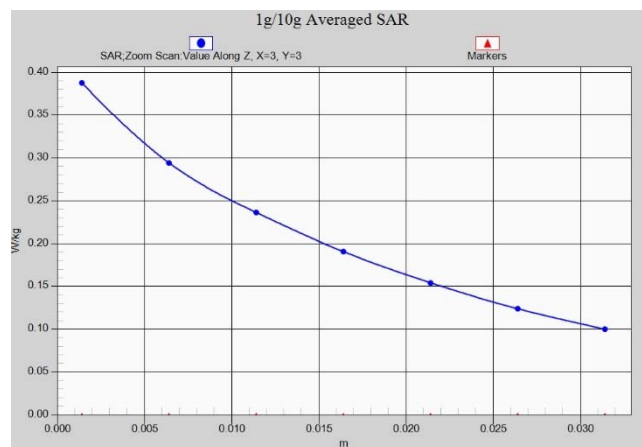
Fig.A.1- 11 Z-Scan at power reference point (CDMA BC0)
