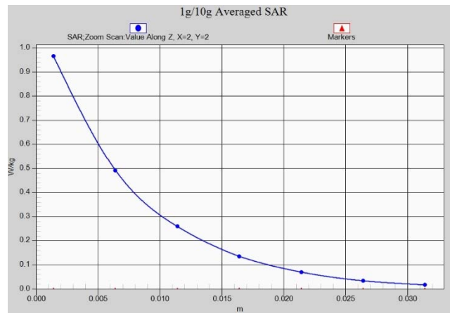
Fig.A.1- 31 Z-Scan at power reference point (LTE band41 PC3)
