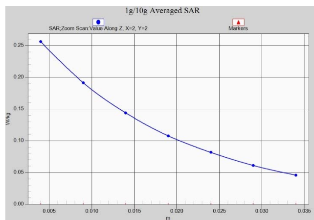
Fig.A.1- 38 Z-Scan at power reference point (LTE band71)
