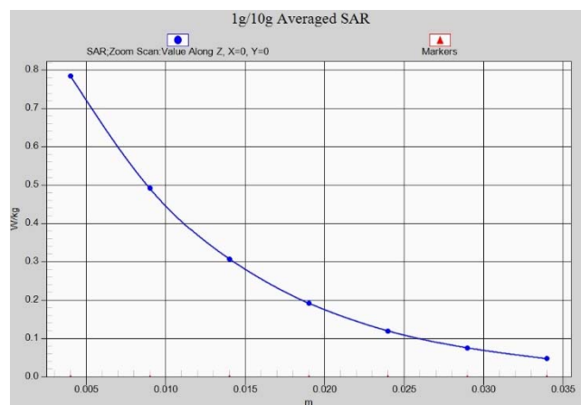
Fig.A.1- 18 Z-Scan at power reference point (LTE band2)
