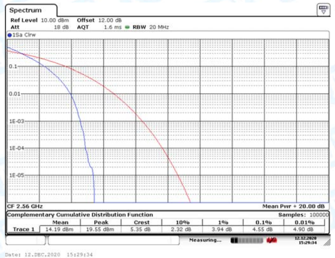
LTE Band 7 20MHz (High Channel)-16QAM
