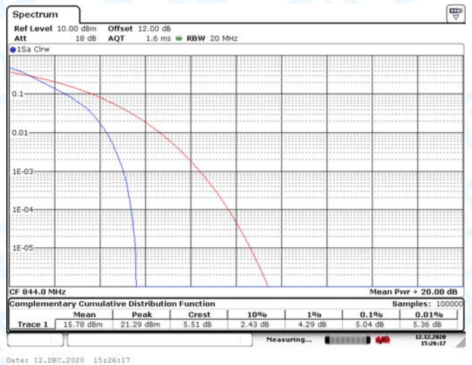
LTE Band 5 10MHz (High Channel)-16QAM
