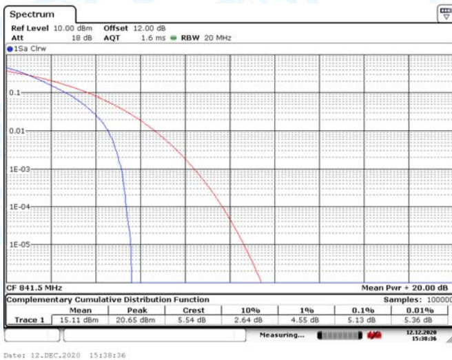
LTE Band 26 15MHz (High Channel)-QPSK
