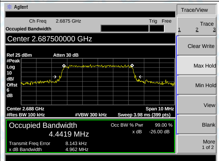
LTE BAND 41 (5MHz 16QAM-High CH)
