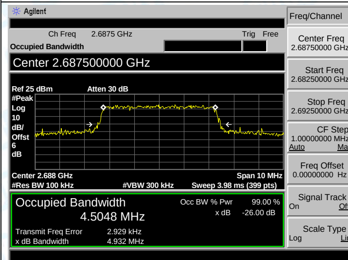
LTE BAND 41 (5MHz QPSK-High CH)
