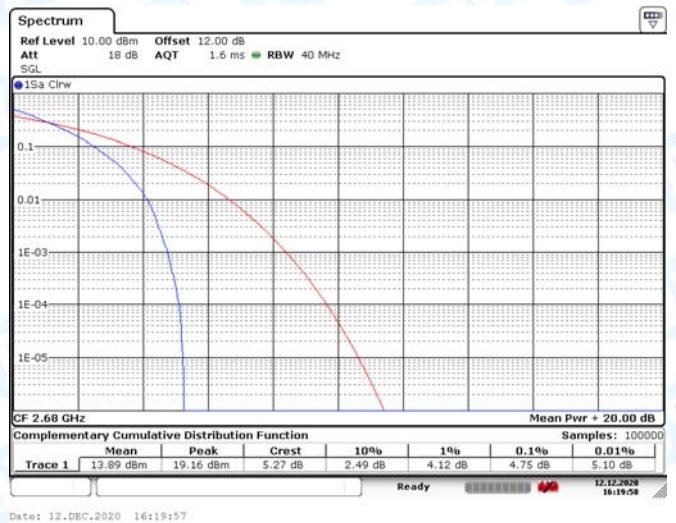
LTE Band 41 20MHz (High Channel)-16QAM
