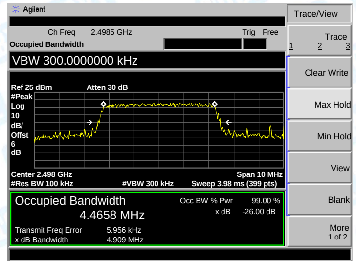
LTE BAND 41 (5MHz 16QAM- Middle CH)
