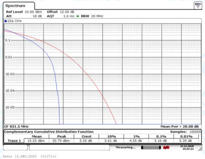
LTE Band 26 15MHz (Middle Channel)-16QAM
