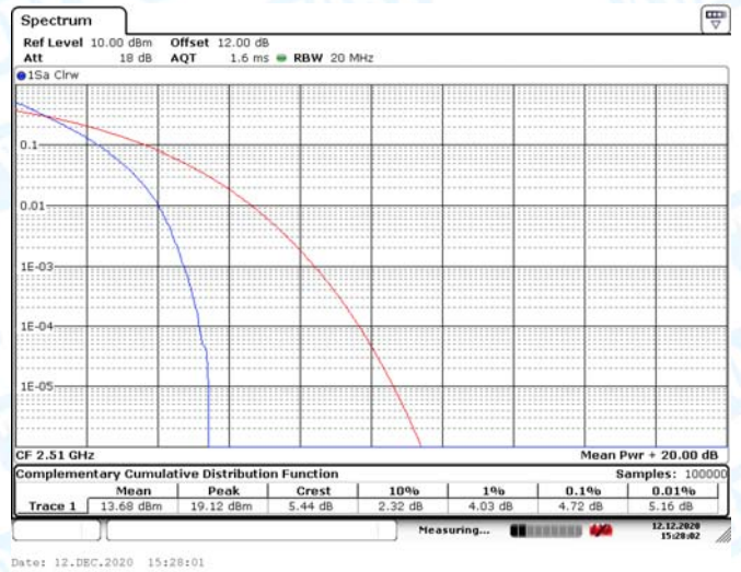
LTE Band 7 20MHz (Middle Channel)-16QAM
