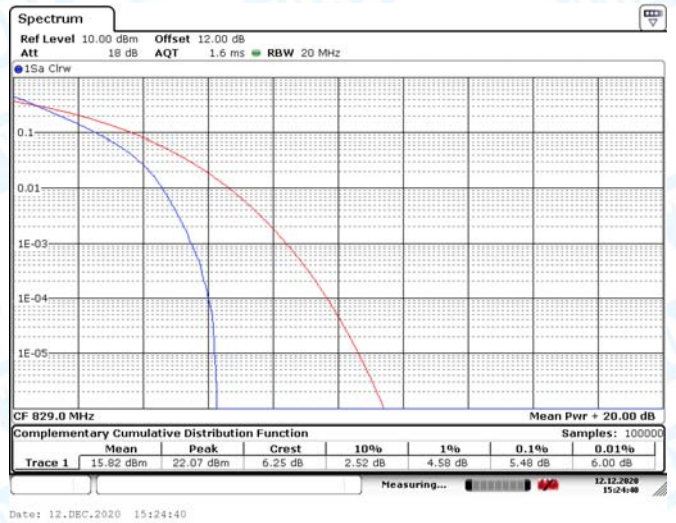
LTE Band 5 10MHz (Middle Channel)-16QAM
