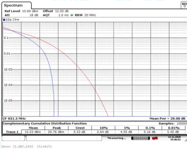
LTE Band 26 15MHz (Middle Channel)-QPSK
