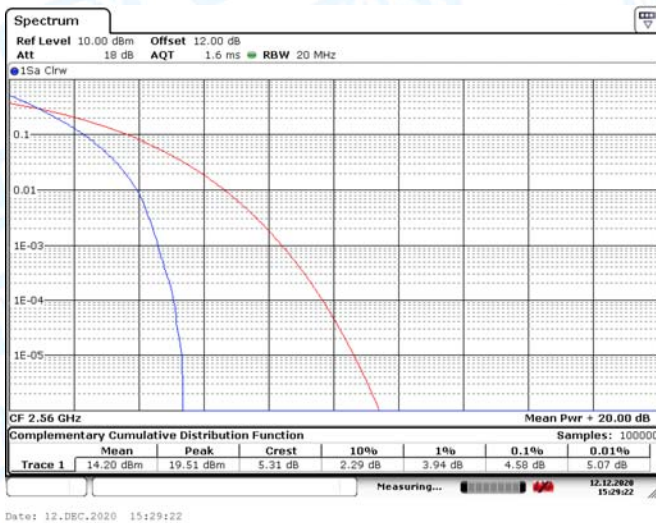
LTE Band 7 20MHz (High Channel)-QPSK
