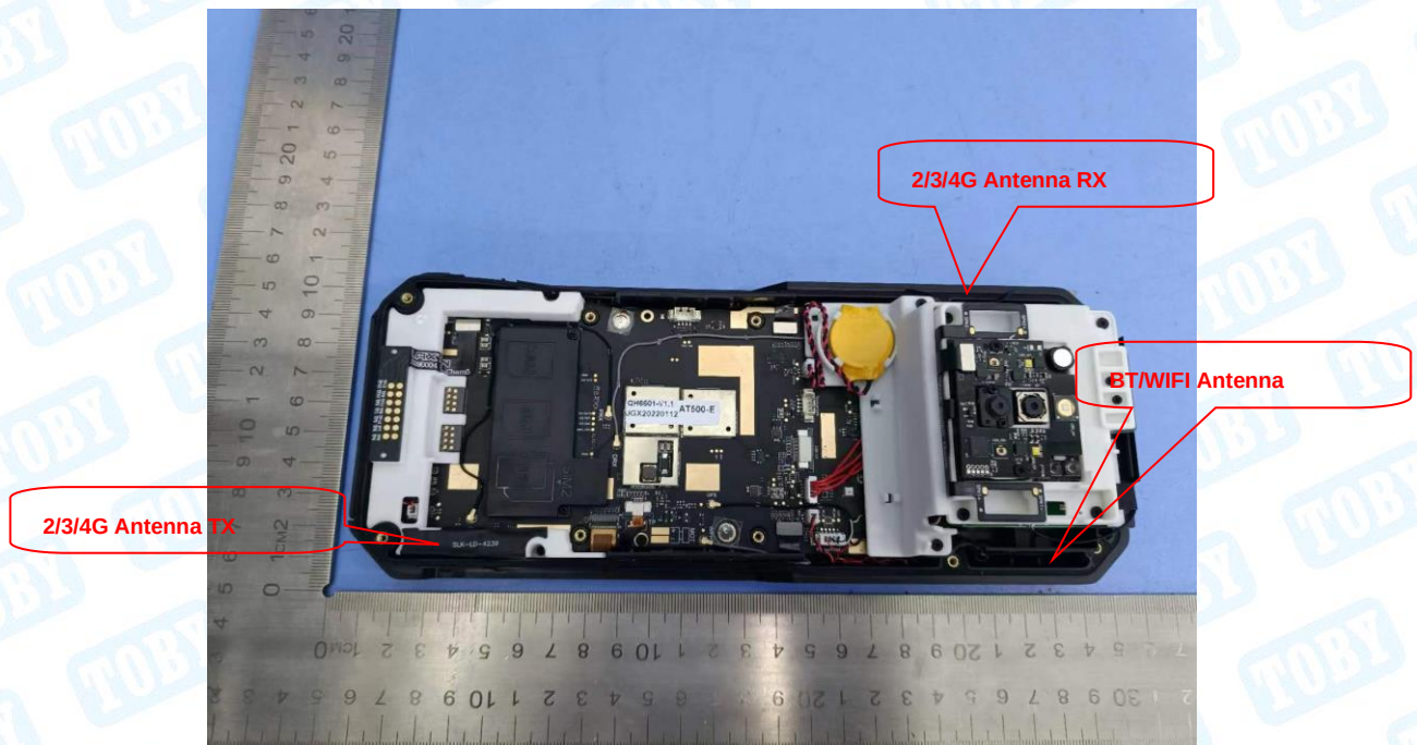
Photo 11 Internal of EUT(DUAL)
