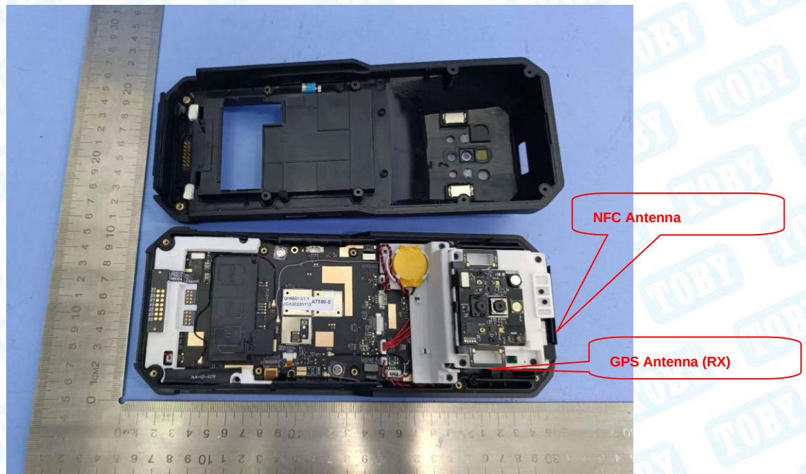
Photo 11 Internal of EUT(DUAL)
