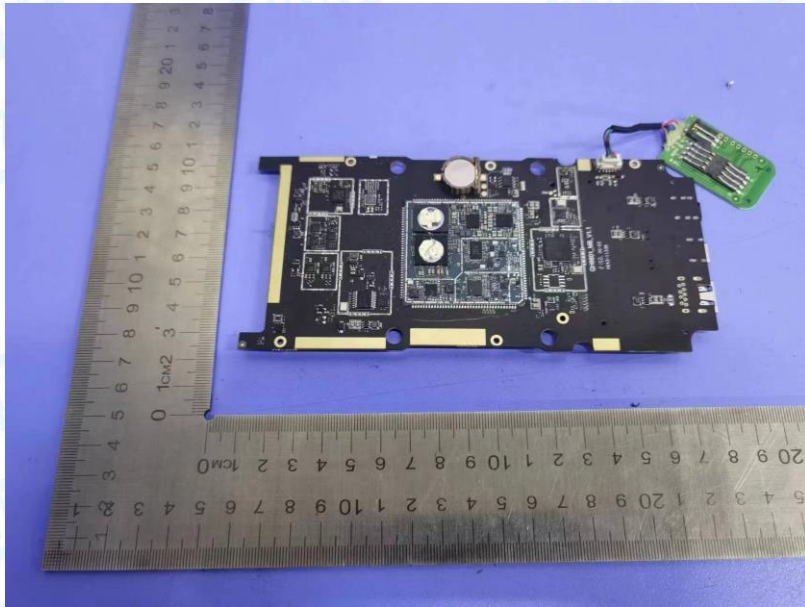
Photo 21 Appearance of PCB
