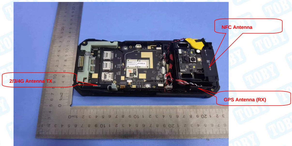
Photo 13 Internal of EUT (SINGLE)
