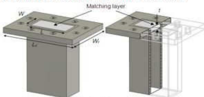
Figure 1: Validation Waveguide Dimensions
