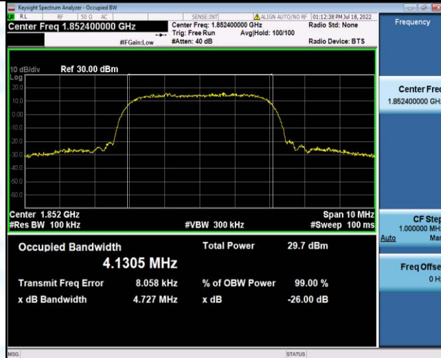
Band2-9262-2
