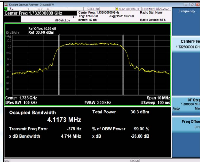
Band4-1413-3
