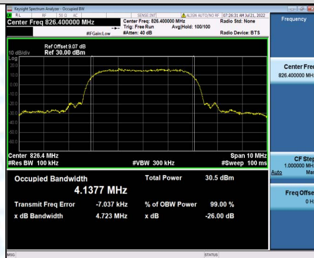
Band5-4132-4
