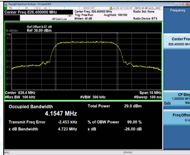
Band5-4132-5
