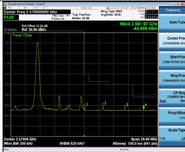
Band7-10MHz-QPSK-21400-1RB#49
