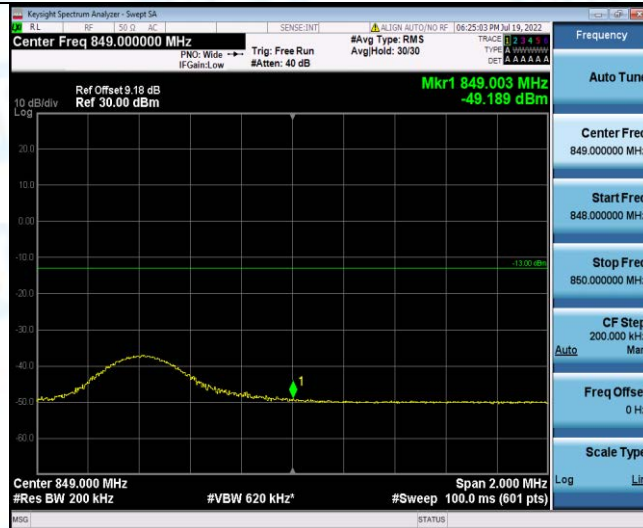
Band5-10MHz-16QAM-20600-1RB#49
