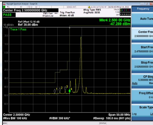
Band7-5MHz-QPSK-20775-25RB#0
