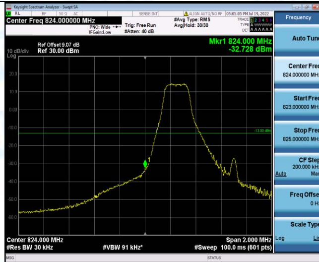
Band5-1.4MHz-16QAM-20407-1RB#5
