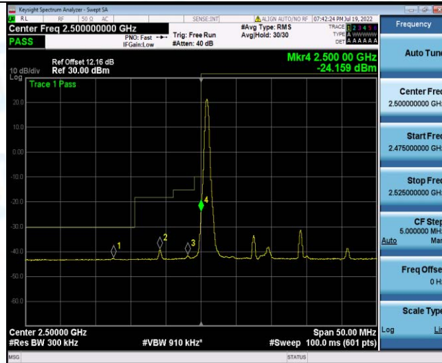
Band7-15MHz-QPSK-20825-1RB#74
