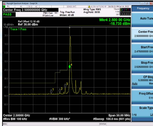
Band7-5MHz-QPSK-20775-1RB#24
