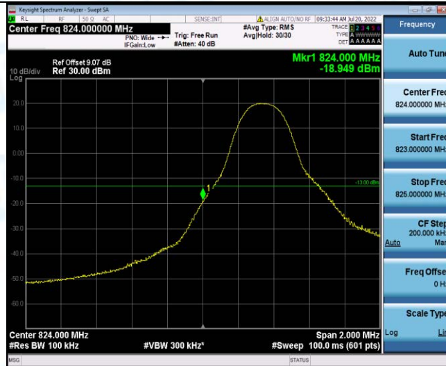
Band26-5MHz-QPSK-26815-1RB#24
