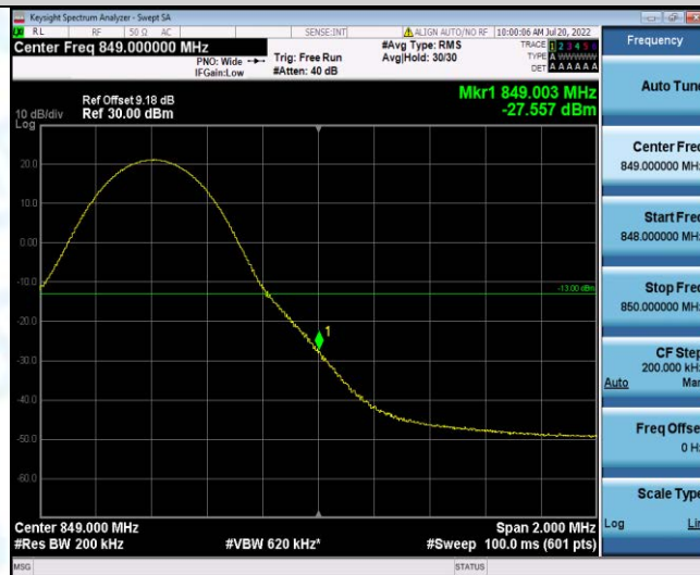
Band26-10MHz-QPSK-26990-50RB#0
