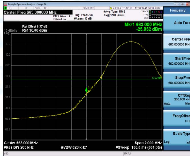
Band71-10MHz-16QAM-133172-1RB#49
