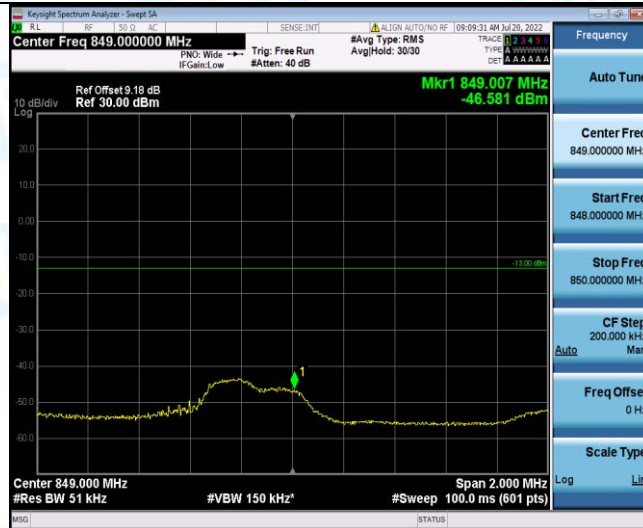
Band26-3MHz-QPSK-27025-1RB#14
