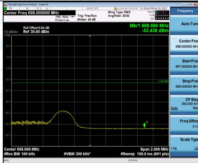
Band71-5MHz-16QAM-133447-1RB#24
