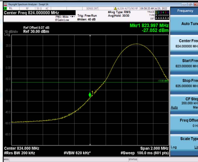
Band26-10MHz-QPSK-26840-1RB#49
