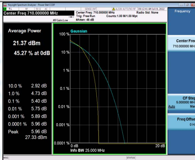
Band17-5MHz-16QAM-23825-1RB#0
