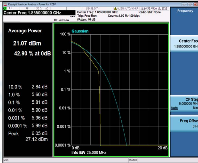
Band25-10MHz-16QAM-26090-50RB#0
