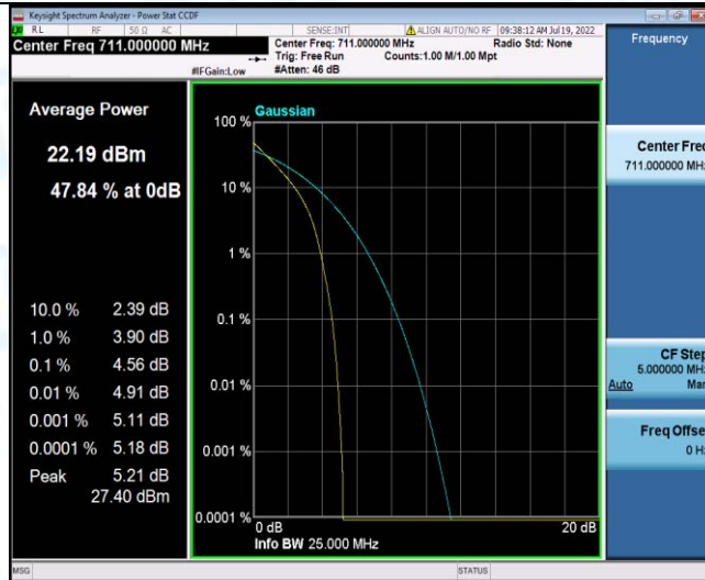
Band17-10MHz-16QAM-23780-1RB#0
