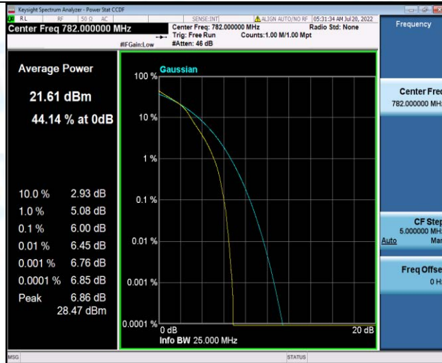
Band13-5MHz-16QAM-23255-1RB#0
