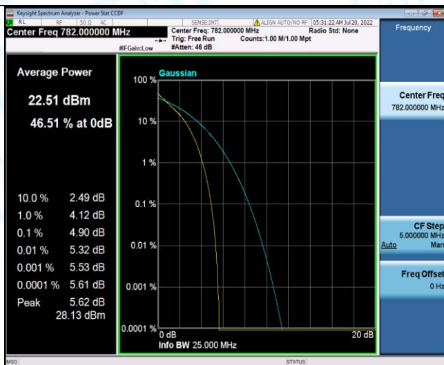
Band13-5MHz-QPSK-23255-1RB#0
