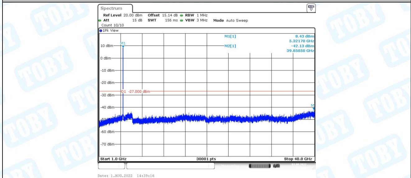
11AC20SISO_Ant1_5320_1000~40000
