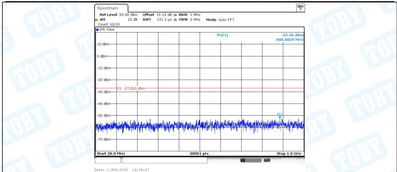
11AC20SISO_Ant1_5320_30~1000
