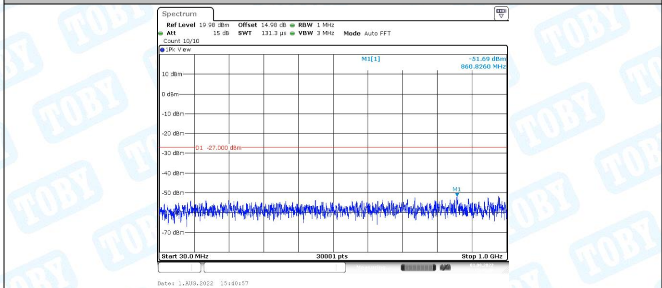
11AC40SISO_Ant1_5190_30~1000
