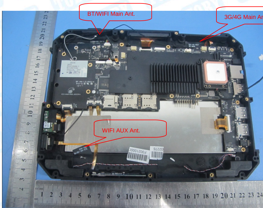
Photo 16 Appearance of PCB
