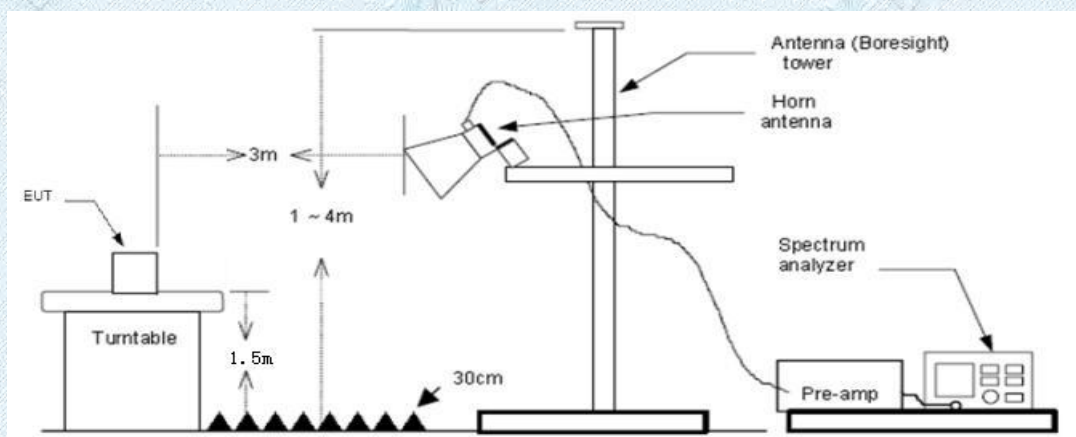
Above 1GHz Test Setup
