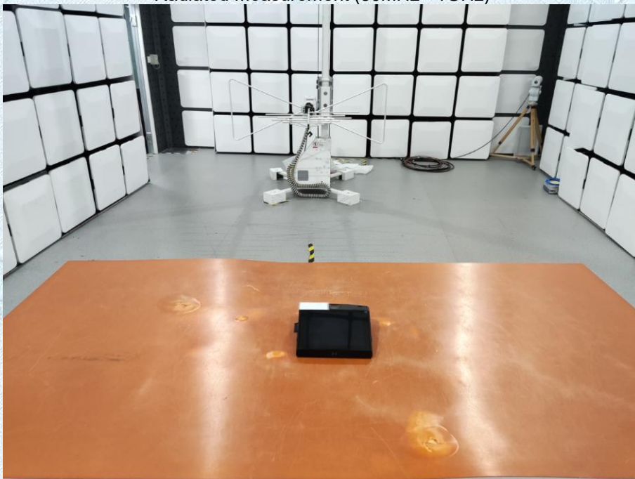
Radiated Measurement (30MHz~ 1GHz)
