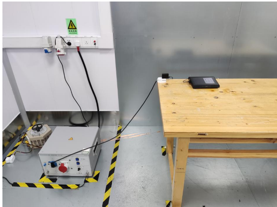
Conducted Emission For AC Mains Power Ports For 2G/3G/4G/WIFI-BT
