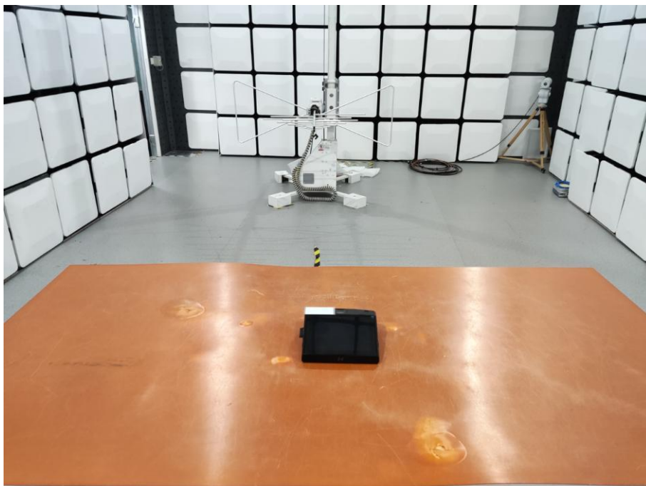
Radiated Emissions (30MHz~1000MHz) For NFC
