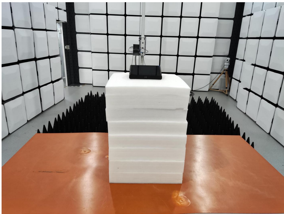
Radiated Emissions (Above 1GHz) For 2G/3G/4G
