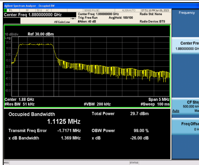
Band2-5MHz-16QAM-18900-6-0-Low-1.1125-1.369-PASS
