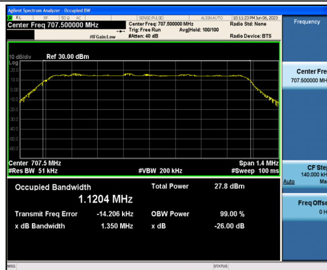
Band12-1.4MHz-16QAM-23095-6-0-Low-1.1204-1.350-PASS
