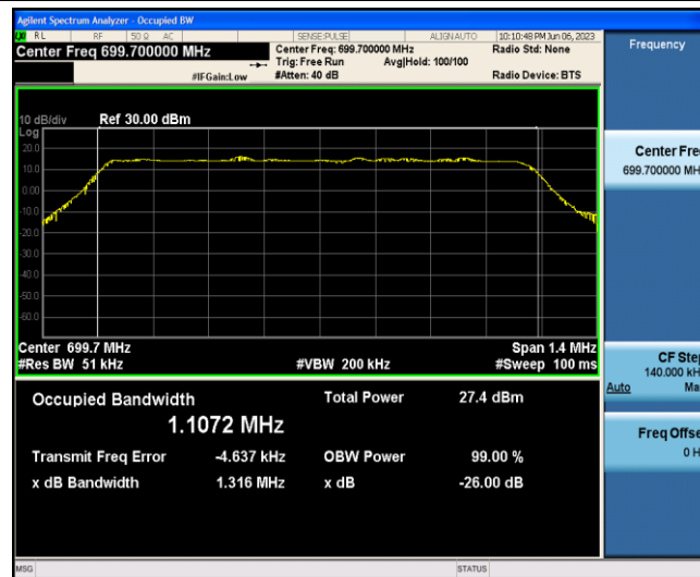
Band12-1.4MHz-16QAM-23017-6-0-Low-1.1072-1.316-PASS
