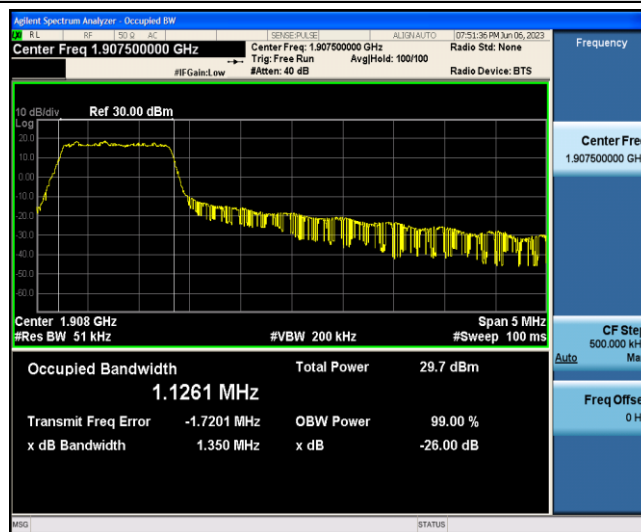
Band2-5MHz-QPSK-19175-6-0-Low-1.1261-1.350-PASS
