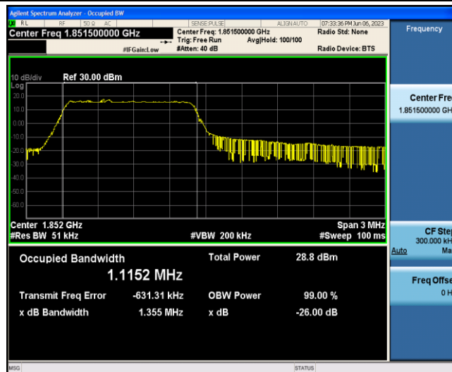
Band2-3MHz-QPSK-18615-6-0-Low-1.1152-1.355-PASS
