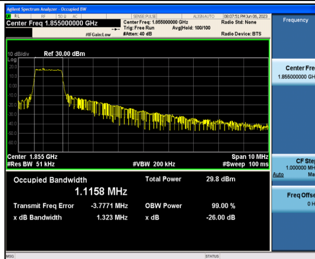
Band2-10MHz-QPSK-18650-6-0-Low-1.1158-1.323-PASS
