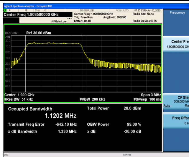
Band2-3MHz-16QAM-19185-6-0-Low-1.1202-1.330-PASS
