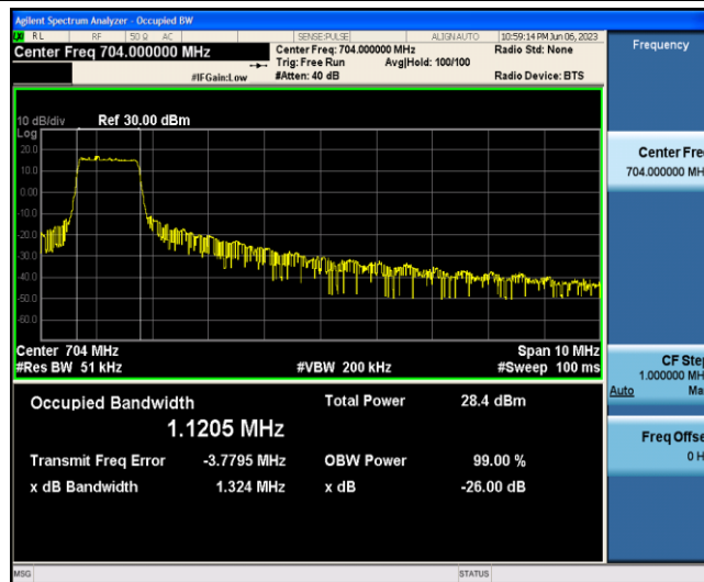
Band12-10MHz-16QAM-23060-6-0-Low-1.1205-1.324-PASS
