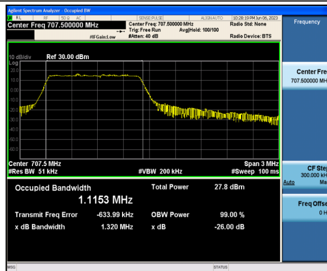
Band12-3MHz-QPSK-23095-6-0-Low-1.1153-1.320-PASS
