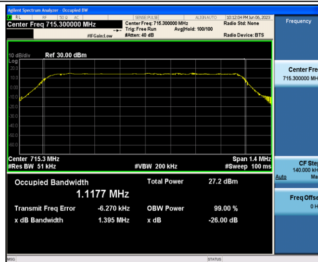
Band12-1.4MHz-16QAM-23173-6-0-Low-1.1177-1.395-PASS
