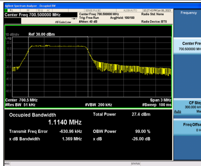
Band12-3MHz-QPSK-23025-6-0-Low-1.1140-1.369-PASS
