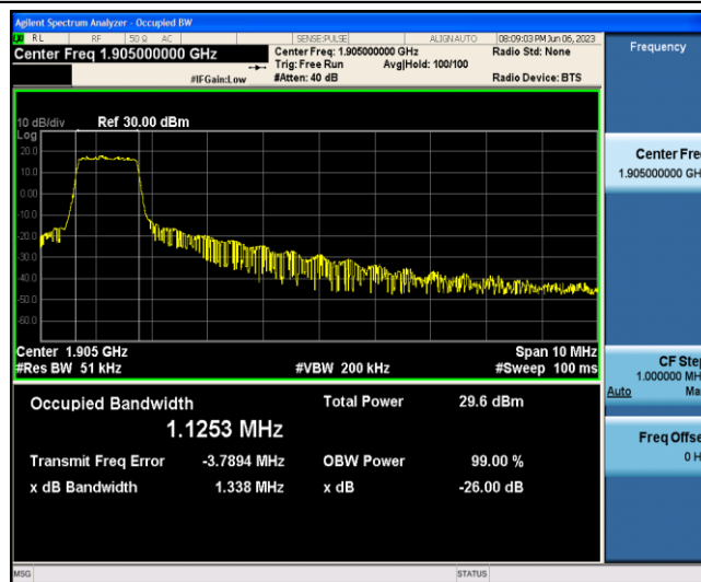
Band2-10MHz-QPSK-19150-6-0-Low-1.1253-1.338-PASS
