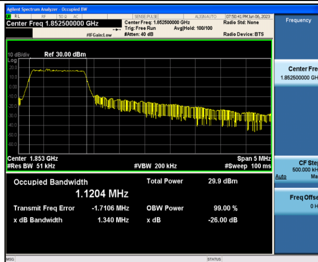
Band2-5MHz-16QAM-18625-6-0-Low-1.1204-1.340-PASS
