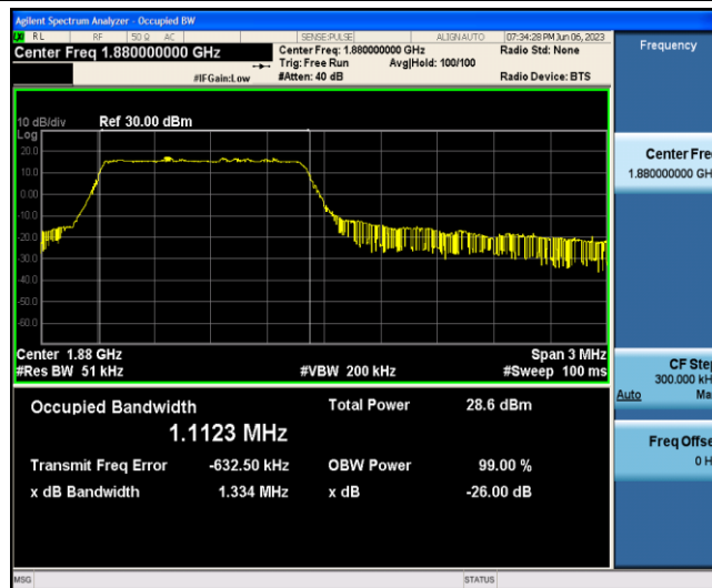
Band2-3MHz-16QAM-18900-6-0-Low-1.1123-1.334-PASS
