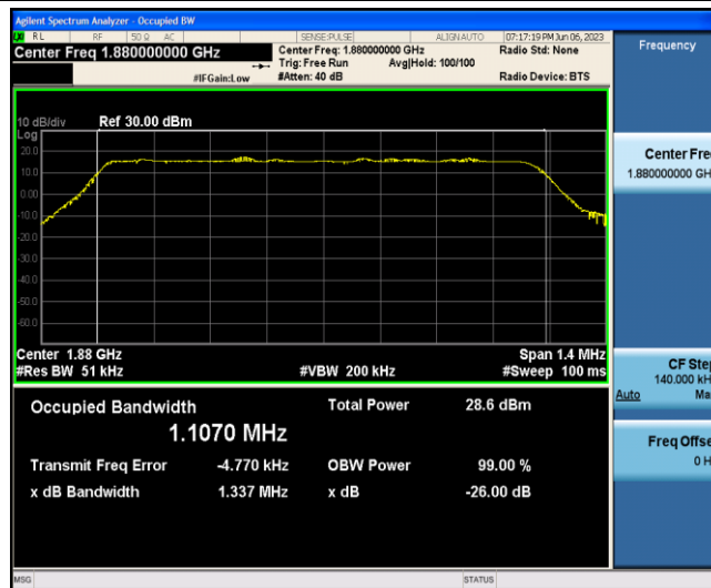
Band2-1.4MHz-16QAM-18900-6-0-Low-1.1070-1.337-PASS
