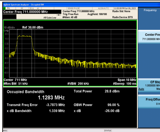
Band12-10MHz-QPSK-23130-6-0-Low-1.1283-1.339-PASS
