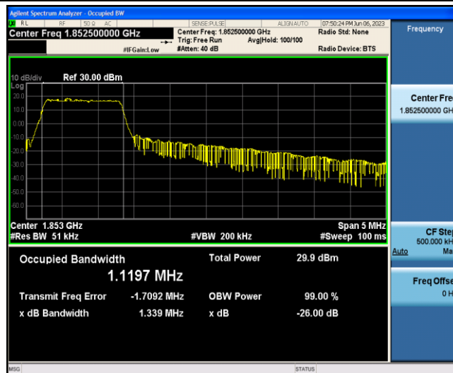
Band2-5MHz-QPSK-18625-6-0-Low-1.1197-1.339-PASS
