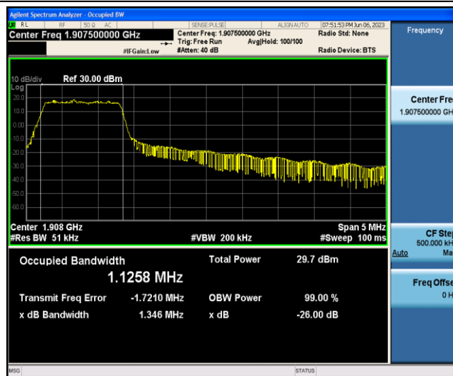
Band2-5MHz-16QAM-19175-6-0-Low-1.1258-1.346-PASS
