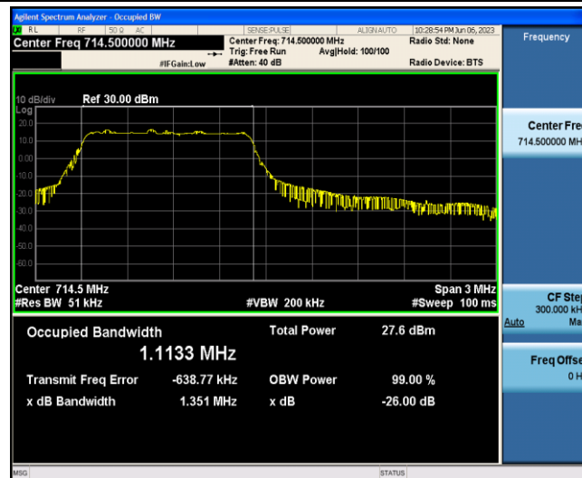
Band12-3MHz-QPSK-23165-6-0-Low-1.1133-1.351-PASS
