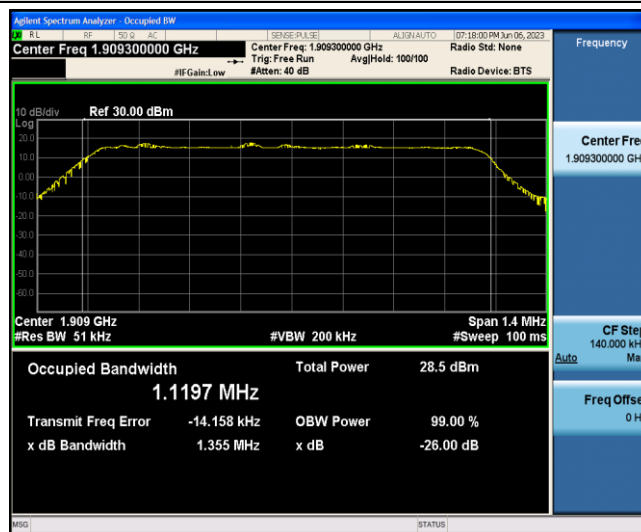
Band2-1.4MHz-16QAM-19193-6-0-Low-1.1197-1.355-PASS
