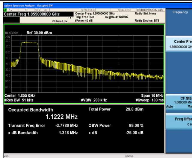
Band2-10MHz-16QAM-18650-6-0-Low-1.1222-1.318-PASS
