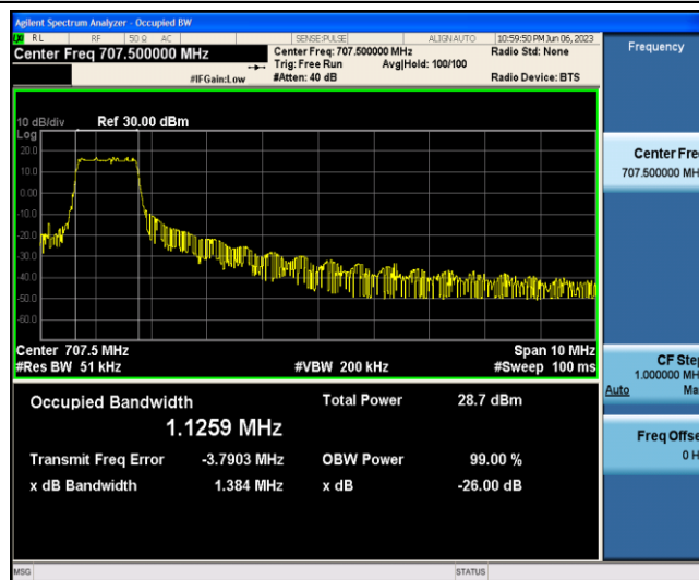
Band12-10MHz-16QAM-23095-6-0-Low-1.1259-1.384-PASS
