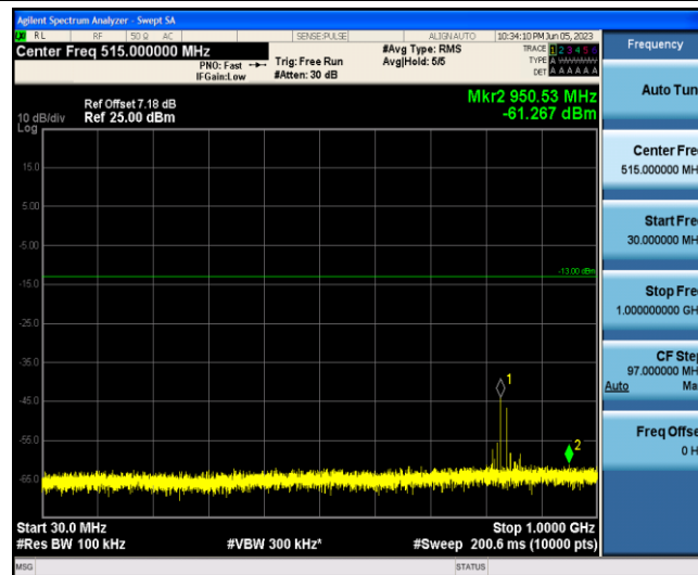
Band5-5MHz-QPSK-20525-1-0-Low-30-1000--61.27-PASS
