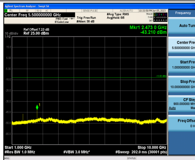
Band5-5MHz-16QAM-20425-1-0-Low-1000-10000--43.21-PASS
