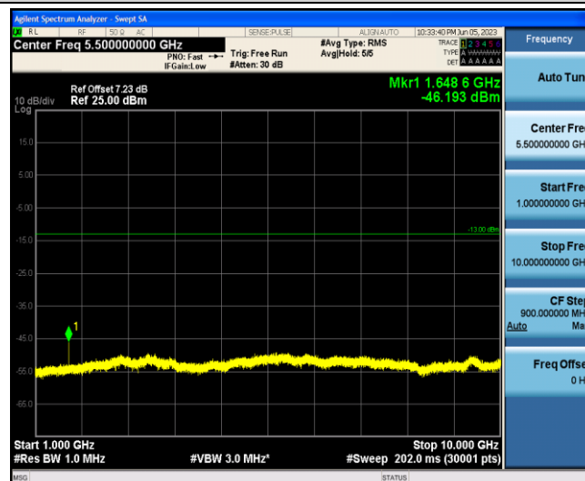
Band5-5MHz-QPSK-20425-1-0-Low-1000-10000--46.19-PASS
