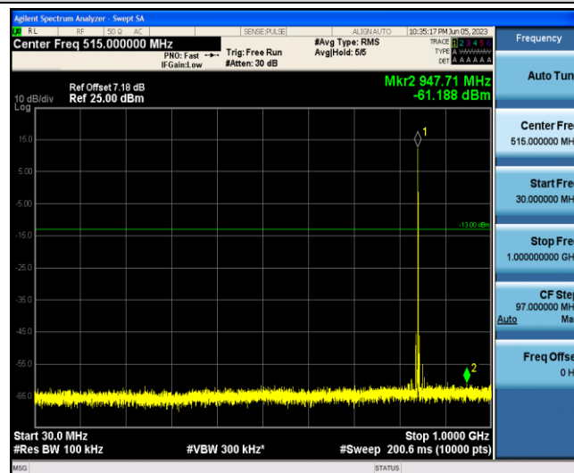
Band5-5MHz-16QAM-20625-1-0-Low-30-1000--61.19-PASS
