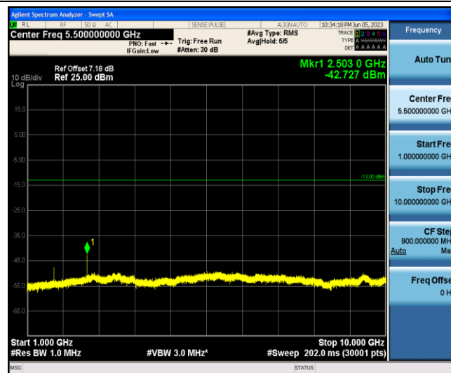
Band5-5MHz-QPSK-20525-1-0-Low-1000-10000--42.73-PASS
