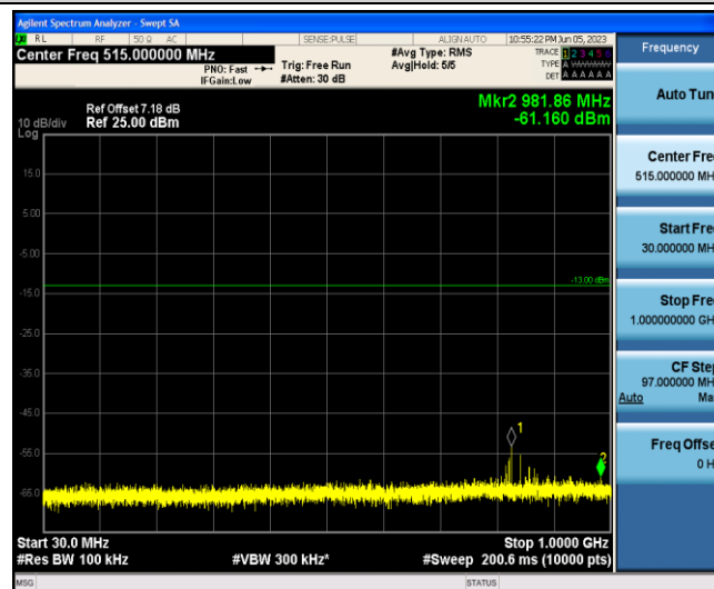
Band5-10MHz-QPSK-20600-1-0-Low-30-1000--61.16-PASS
