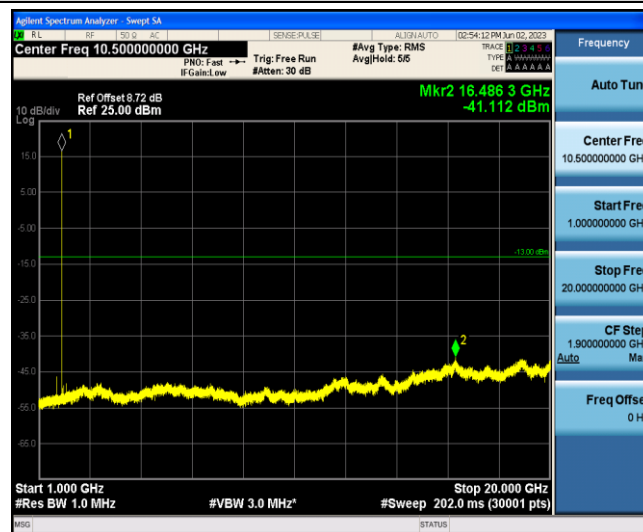
Band2-5MHz-QPSK-18625-1-0-Low-1000-20000--41.11-PASS
