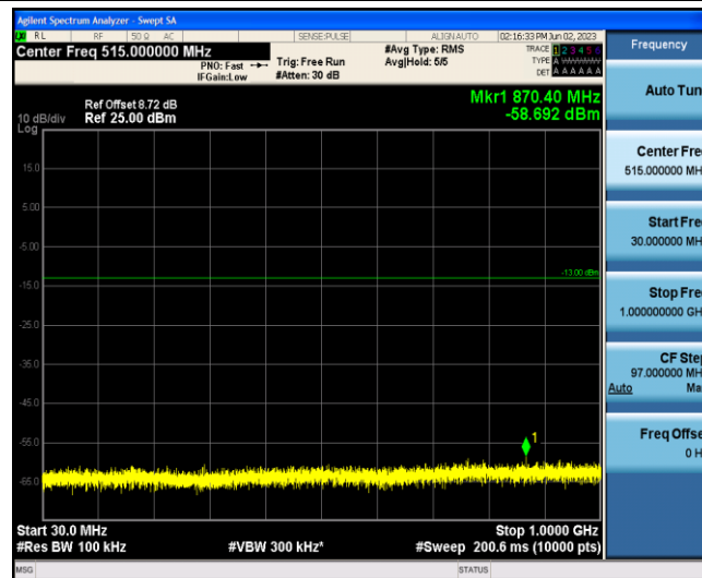
Band2-1.4MHz-16QAM-18607-1-0-Low-30-1000--58.69-PASS
