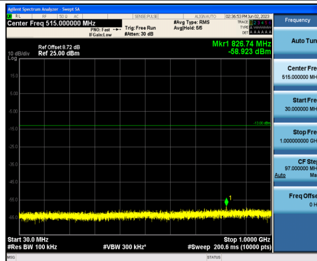
Band2-3MHz-16QAM-18615-1-0-Low-30-1000--58.92-PASS
