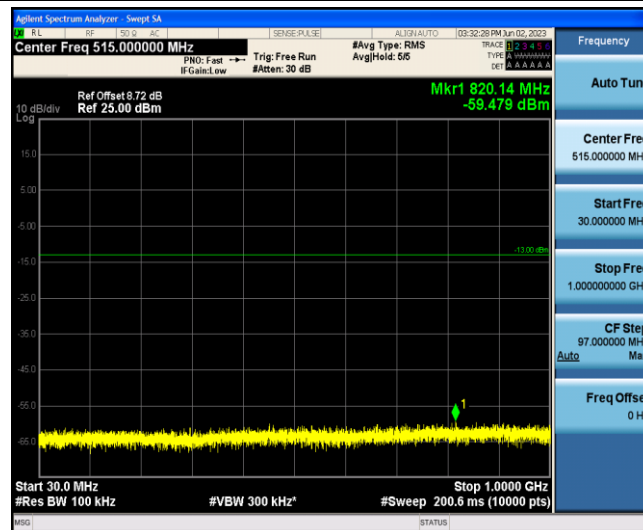
Band2-15MHz-16QAM-18675-1-0-Low-30-1000--59.48-PASS
