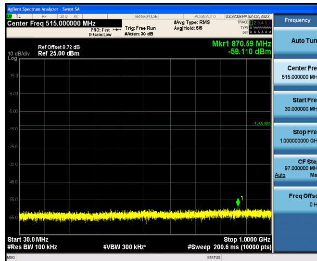
Band2-15MHz-QPSK-18675-1-0-Low-30-1000--59.11-PASS
