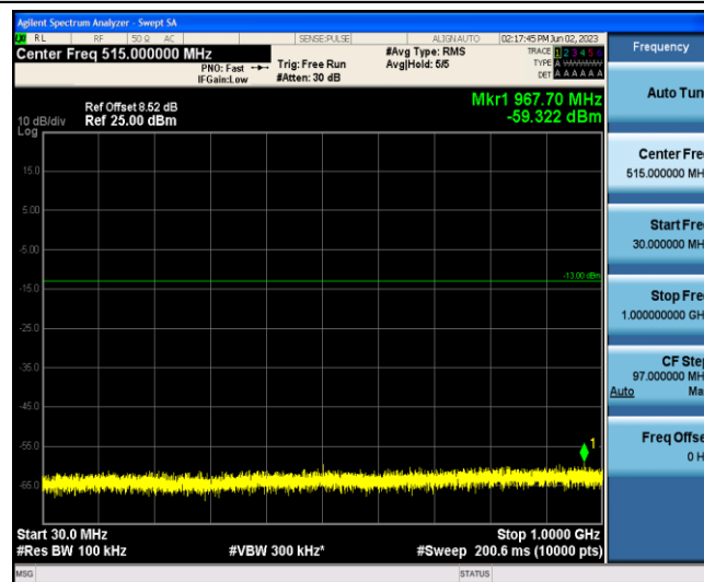
Band2-1.4MHz-QPSK-19193-1-0-Low-30-1000--59.32-PASS
