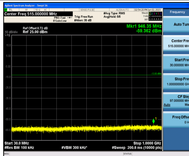
Band2-5MHz-16QAM-18625-1-0-Low-30-1000--59.36-PASS
