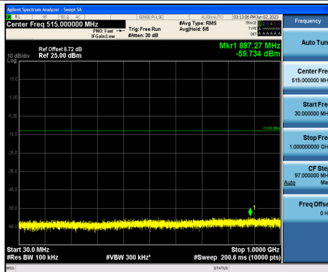
Band2-10MHz-QPSK-18650-1-0-Low-30-1000--59.73-PASS
