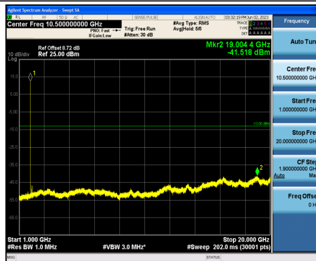
Band2-15MHz-QPSK-18675-1-0-Low-1000-20000--41.52-PASS
