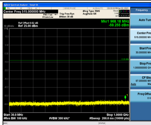
Band2-15MHz-QPSK-19125-1-0-Low-30-1000--59.26-PASS
