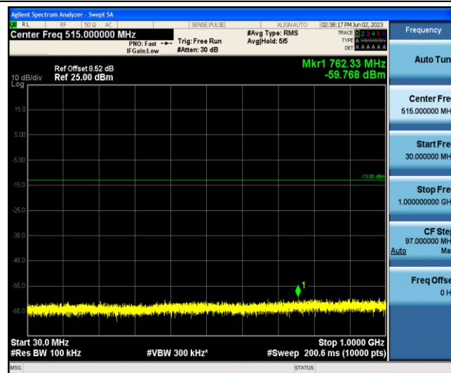
Band2-3MHz-16QAM-19185-1-0-Low-30-1000--59.77-PASS
