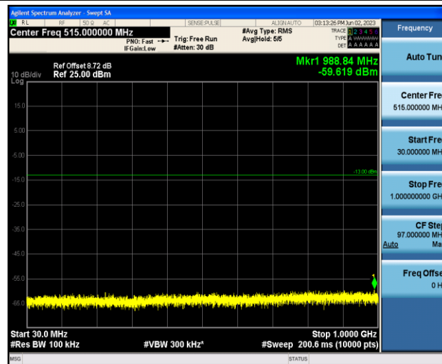
Band2-10MHz-16QAM-18650-1-0-Low-30-1000--59.62-PASS
