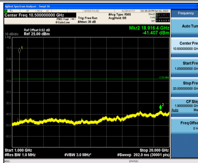
Band2-3MHz-16QAM-19185-1-0-Low-1000-20000--41.41-PASS
