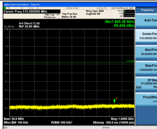
Band2-3MHz-16QAM-18900-1-0-Low-30-1000--59.46-PASS
