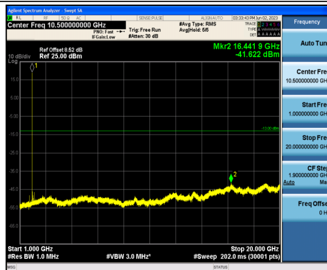
Band2-15MHz-QPSK-19125-1-0-Low-1000-20000--41.62-PASS
