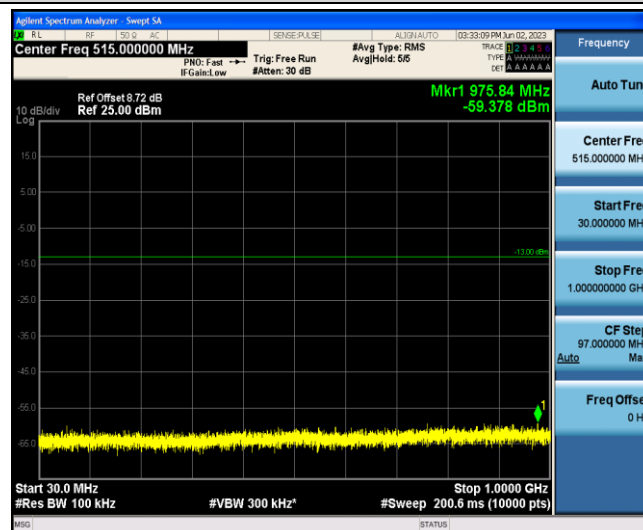
Band2-15MHz-16QAM-18900-1-0-Low-30-1000--59.38-PASS
