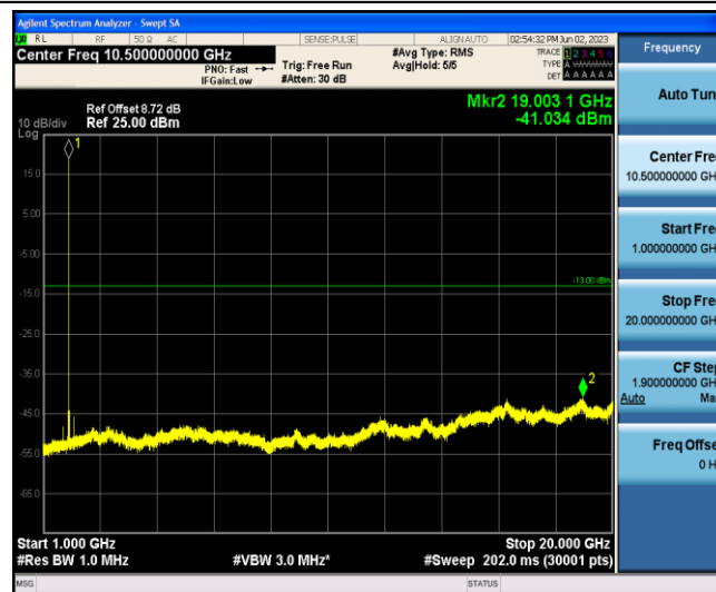
Band2-5MHz-16QAM-18625-1-0-Low-1000-20000--41.03-PASS
