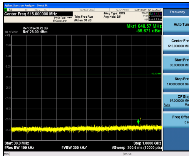
Band2-5MHz-QPSK-18625-1-0-Low-30-1000--59.67-PASS
