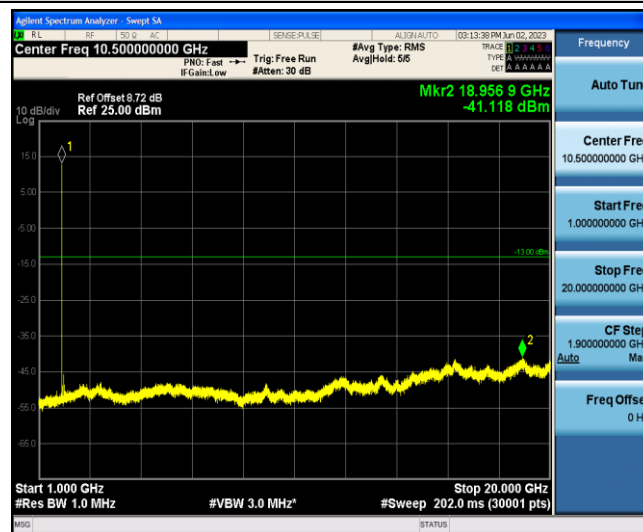
Band2-10MHz-16QAM-18650-1-0-Low-1000-20000--41.12-PASS
