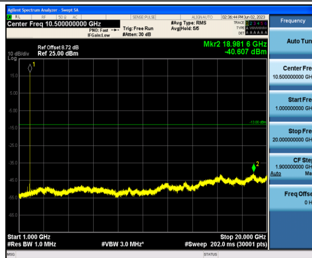
Band2-3MHz-QPSK-18615-1-0-Low-1000-20000--40.61-PASS
