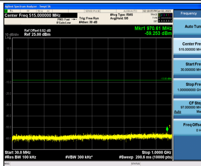
Band2-1.4MHz-16QAM-19193-1-0-Low-30-1000--59.25-PASS
