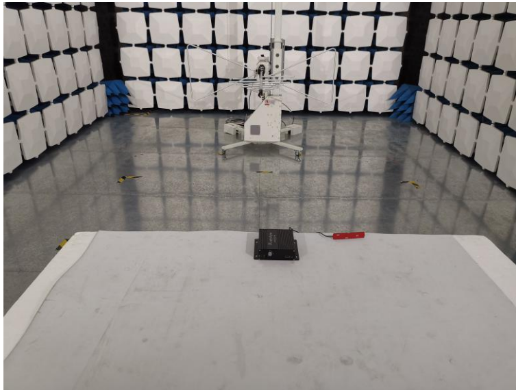
Blow 1GHz for radiated emission test setup
