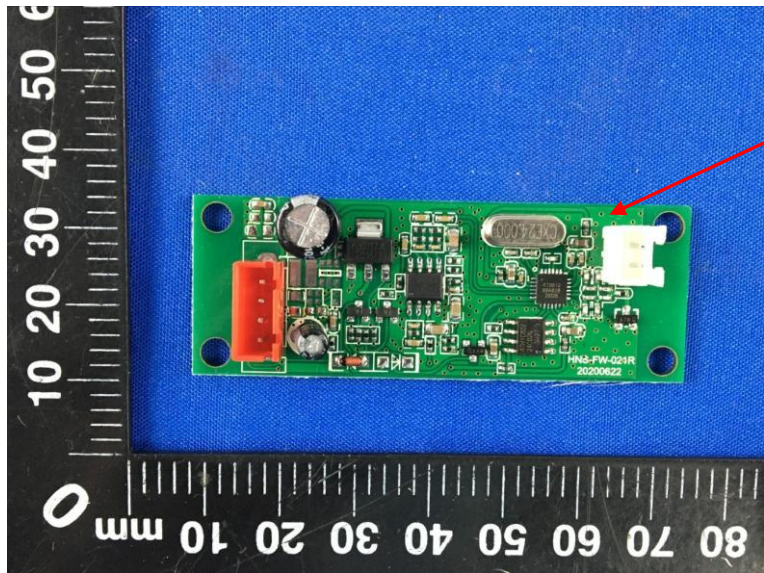
Wireless Microphone RX modular
