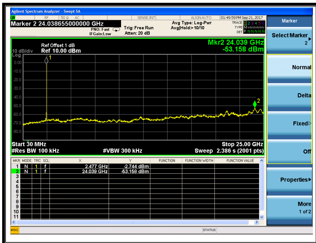
(Plot C: Channel = 16, 30MHz to 25GHz @ GFSK Mode)
