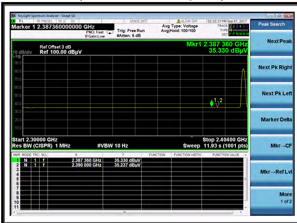
(Plot A2: Channel = 1 AVERAGE @ GFSK)
