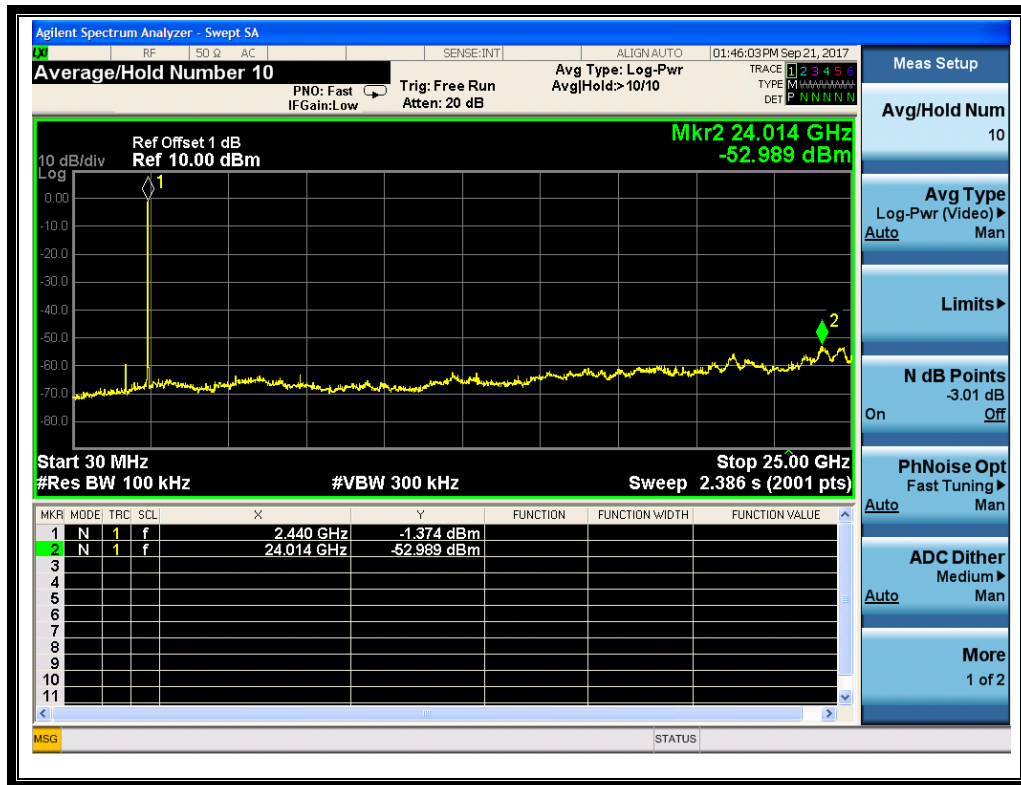
(Plot B: Channel = 9, 30MHz to 25GHz @ GFSK Mode)
