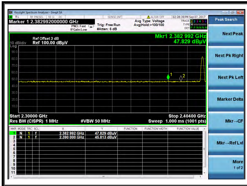
(Plot A1: Channel = 1 PEAK @ GFSK)
