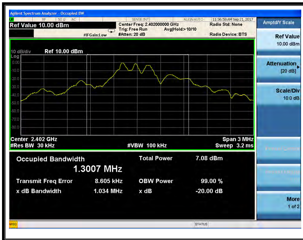
(Plot A: Channel = 1 @ GFSK)
