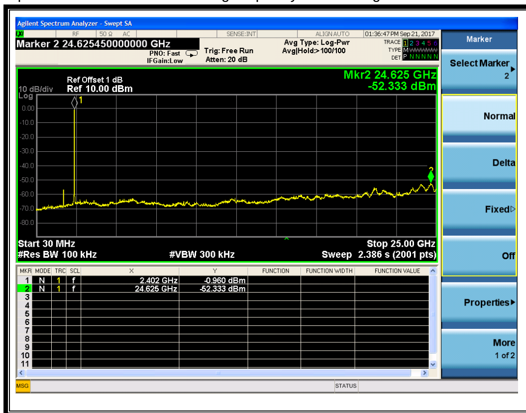
(Plot A: Channel = 1, 30MHz to 25GHz @ GFSK Mode)
