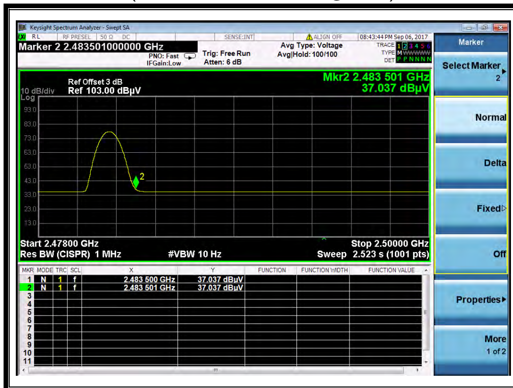
(Plot B2: Channel = 16 AVERAGE @ GFSK)
