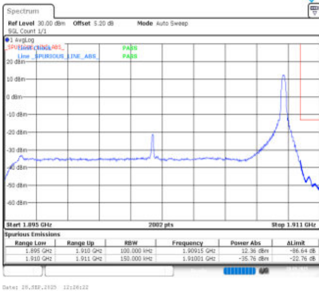
Band2-15MHz-16QAM-19125-1RB#74-PASS
