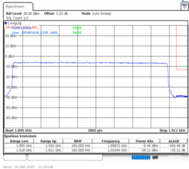
Band2-15MHz-16QAM-19125-75RB#0-PASS
