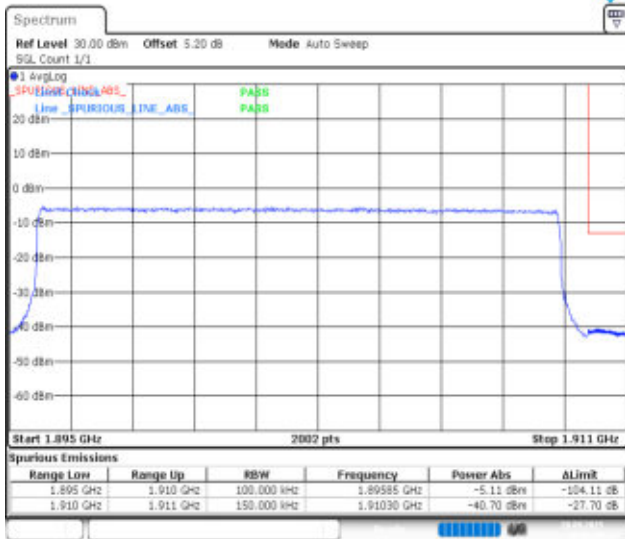
Band2-15MHz-QPSK-19125-75RB#0-PASS
