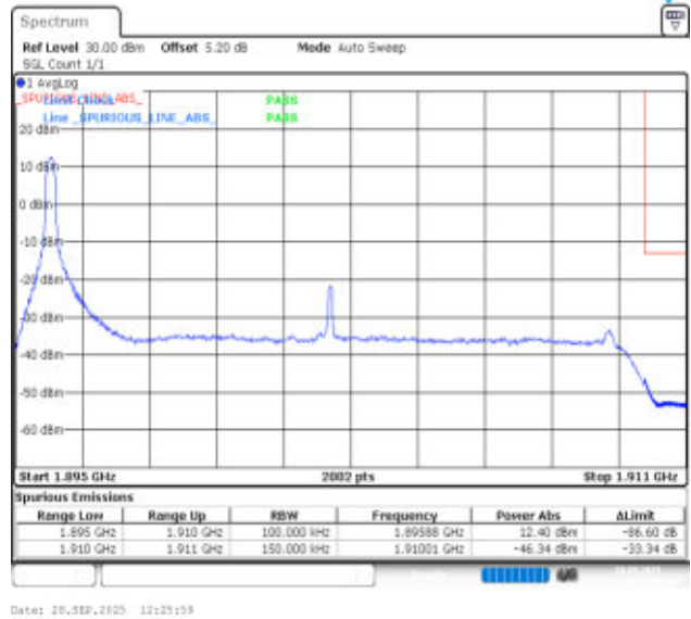
Band2-15MHz-16QAM-19125-1RB#0-PASS
