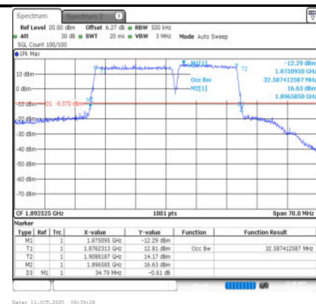
2-2-20MHz-15MHz-16QAM-16QAM-18951-19122-100RB#0-75RB#0-PASS
