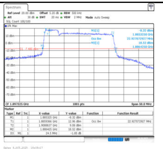
2-2-5MHz-20MHz-16QAM-16QAM-18983-19100-25RB#0-100RB#0-PASS
