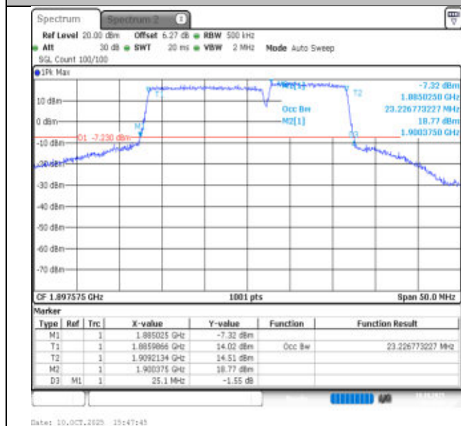
2-2-15MHz-10MHz-QPSK-QPSK-19027-19147-75RB#0-50RB#0-PASS
