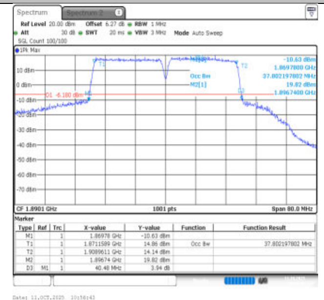
2-2-20MHz-20MHz-16QAM-16QAM-18902-19100-100RB#0-100RB#0-PASS
