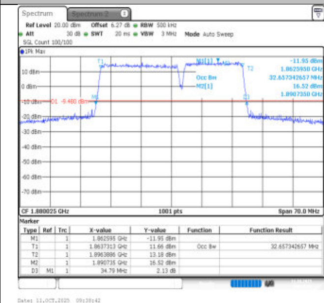
2-2-20MHz-15MHz-16QAM-16QAM-18826-18997-100RB#0-75RB#0-PASS
