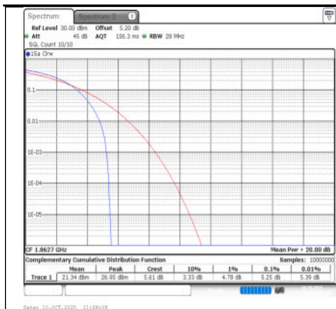
2-2-10MHz-20MHz-QPSK-QPSK-18655-18799-50RB#0- 100RB#0-PASS
