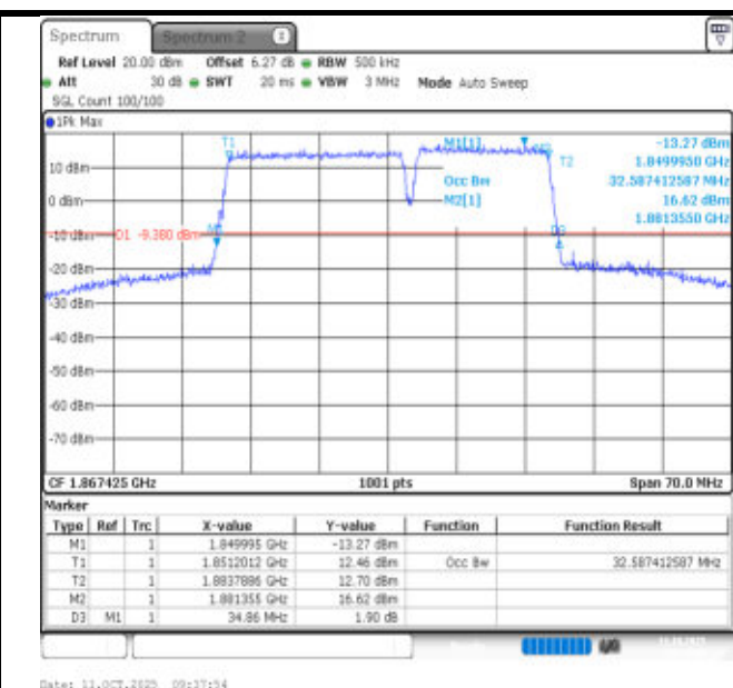
2-2-20MHz-15MHz-16QAM-16QAM-18700-18871-100RB#0-75RB#0-PASS
