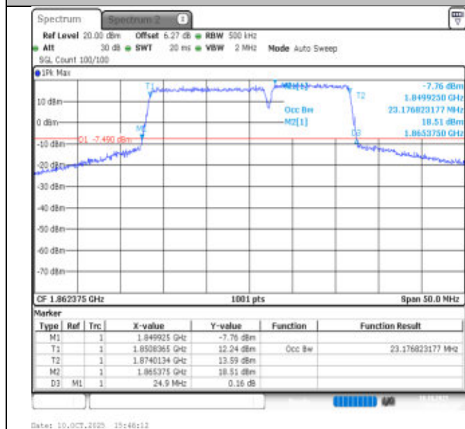
2-2-15MHz-10MHz-QPSK-QPSK-18675-18795-75RB#0-50RB#0-PASS
