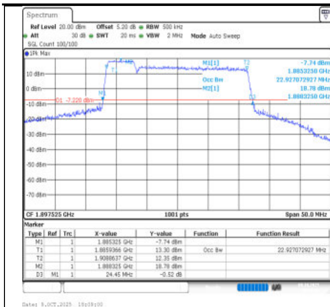
2-2-5MHz-20MHz-QPSK-QPSK-18983-19100-25RB#0-100RB#0-PASS
