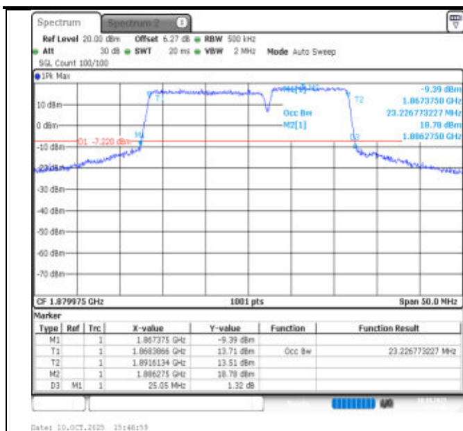
2-2-15MHz-10MHz-QPSK-QPSK-18851-18971-75RB#0-50RB#0-PASS
