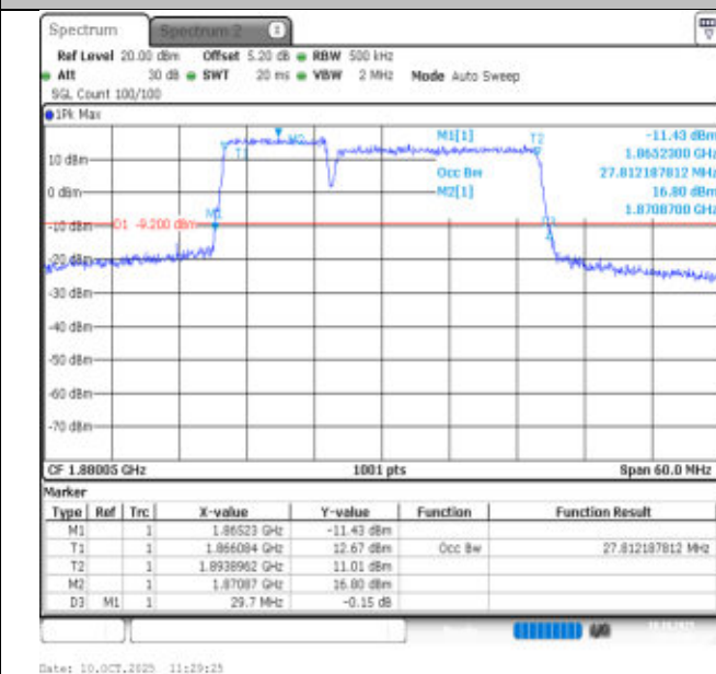
2-2-10MHz-20MHz-16QAM-16QAM-18806-18950-50RB#0-100RB#0-PASS
