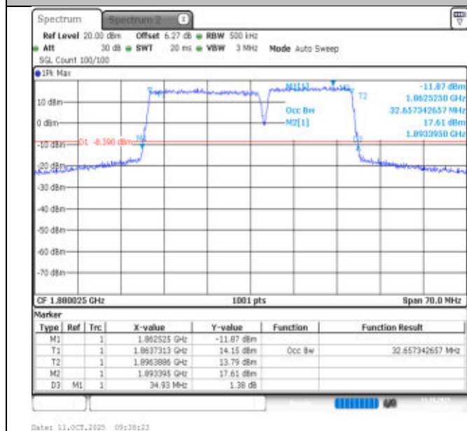
2-2-20MHz-15MHz-QPSK-QPSK-18826-18997-100RB#0-75RB#0-PASS
