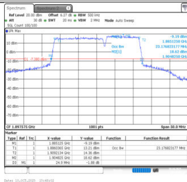
2-2-15MHz-10MHz-16QAM-16QAM-19027-19147-75RB#0-50RB#0-PASS
