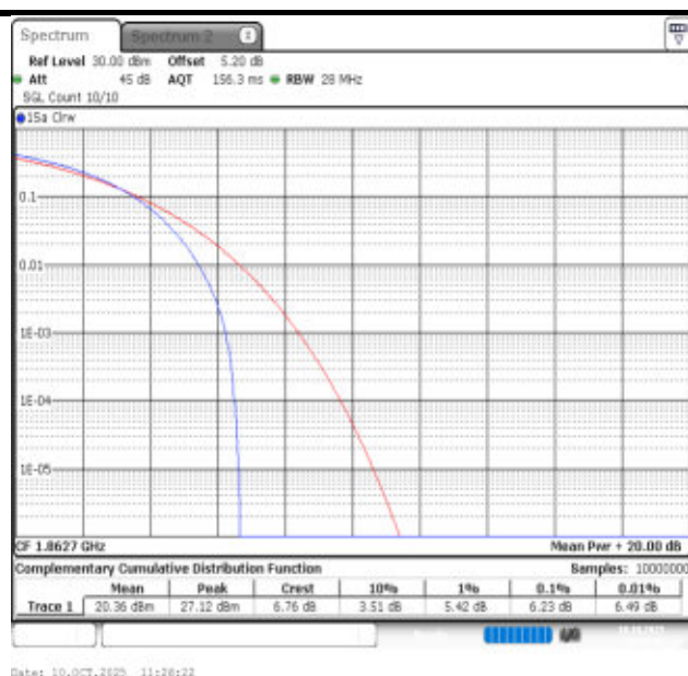
2-2-10MHz-20MHz-16QAM-16QAM-18655-18799-50RB#0- 100RB#0-PASS
