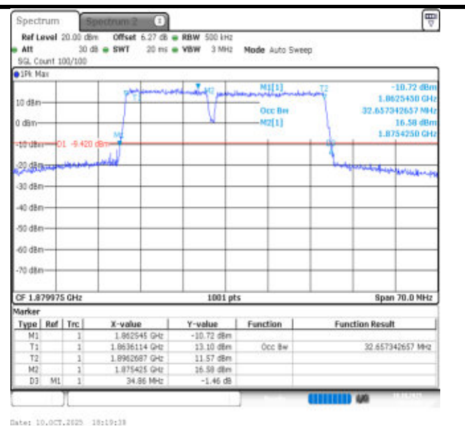
2-2-15MHz-20MHz-16QAM-16QAM-18803-18974-75RB#0-100RB#0-PASS
