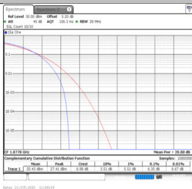
2-2-10MHz-20MHz-16QAM-16QAM-18806-18950-50RB#0- 100RB#0-PASS
