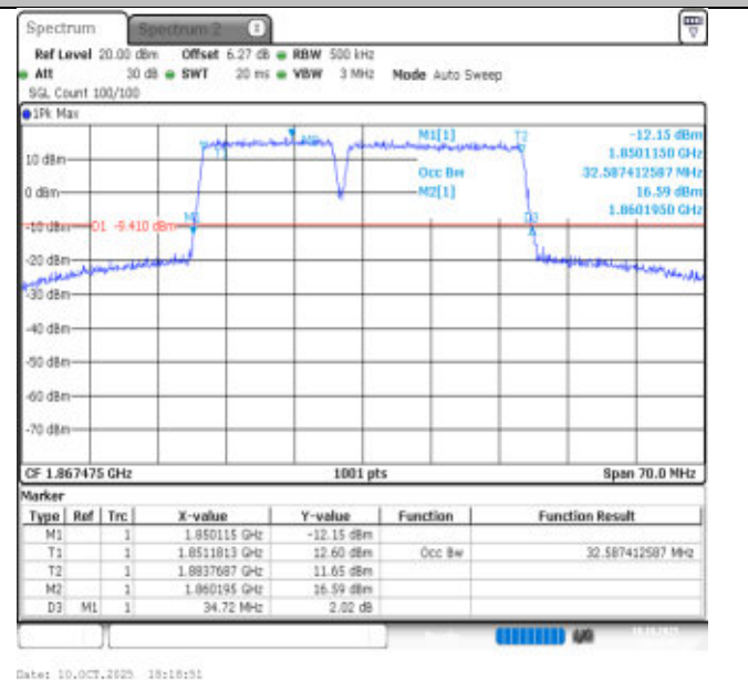
2-2-15MHz-20MHz-16QAM-16QAM-18678-18849-75RB#0-100RB#0-PASS
