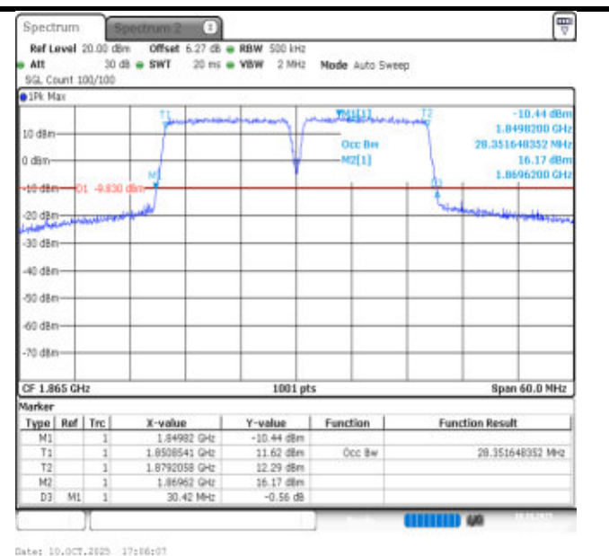
2-2-15MHz-15MHz-16QAM-16QAM-18675-18825-75RB#0-75RB#0-PASS
