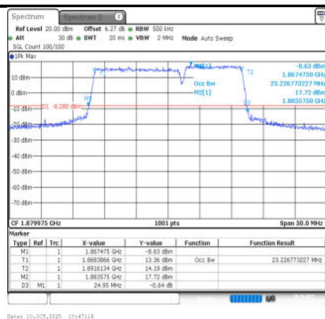
2-2-15MHz-10MHz-16QAM-16QAM-18851-18971-75RB#0-50RB#0-PASS
