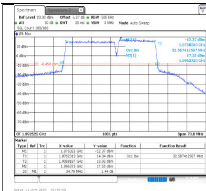
2-2-20MHz-15MHz-QPSK-QPSK-18951-19122-100RB#0-75RB#0-PASS
