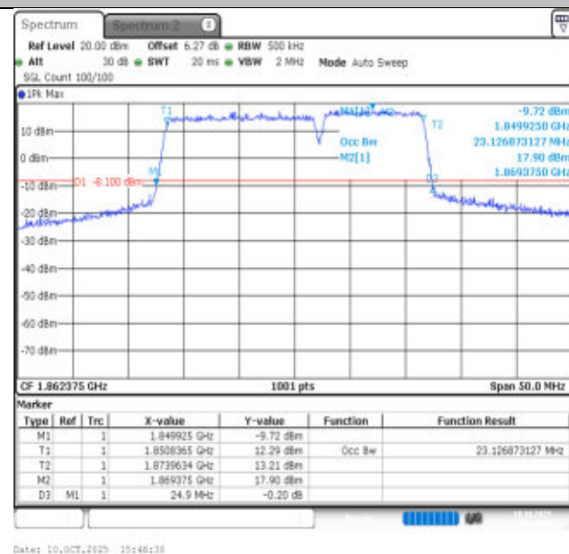
2-2-15MHz-10MHz-16QAM-16QAM-18675-18795-75RB#0-50RB#0-PASS
