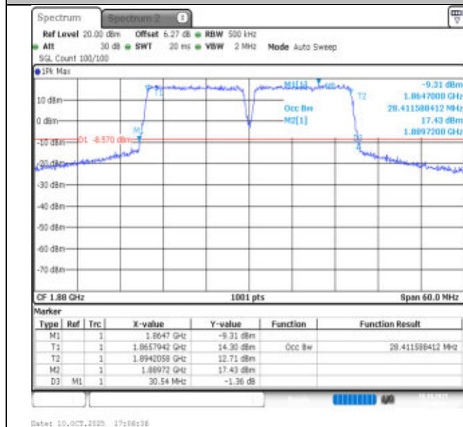
2-2-15MHz-15MHz-QPSK-QPSK-18825-18975-75RB#0-75RB#0-PASS
