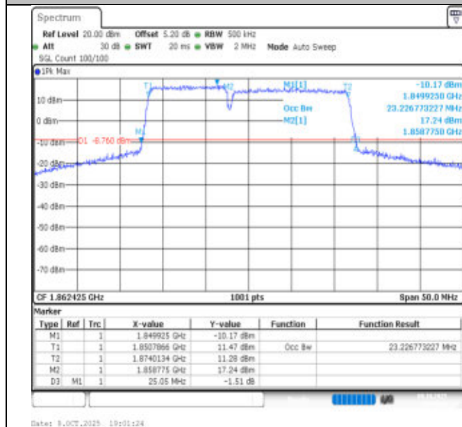
2-2-10MHz-15MHz-QPSK-QPSK-18653-18773-50RB#0-75RB#0-PASS
