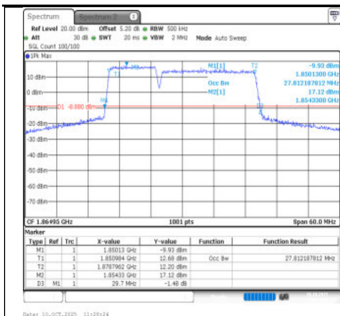
2-2-10MHz-20MHz-QPSK-QPSK-18655-18799-50RB#0-100RB#0-PASS
