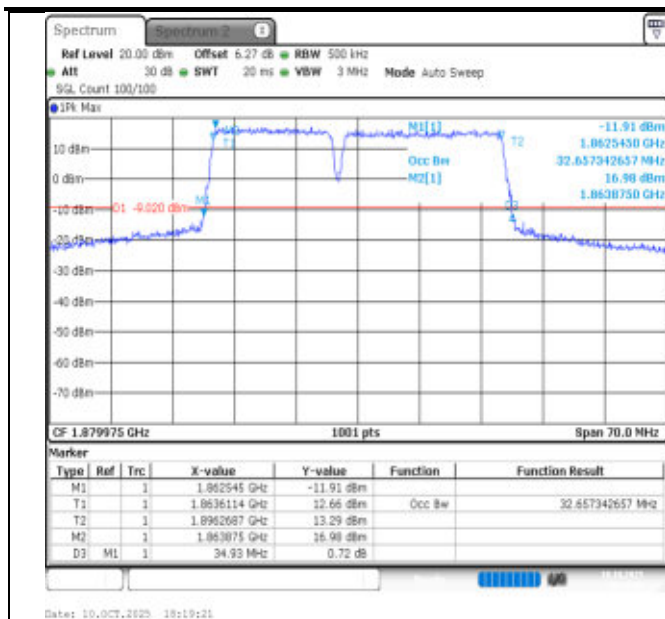
2-2-15MHz-20MHz-QPSK-QPSK-18803-18974-75RB#0-100RB#0-PASS
