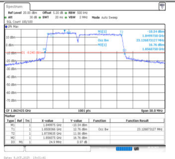
2-2-10MHz-15MHz-16QAM-16QAM-18653-18773-50RB#0-75RB#0-PASS
