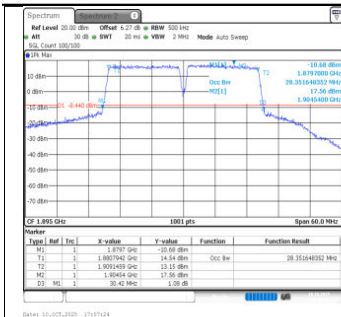
2-2-15MHz-15MHz-QPSK-QPSK-18975-19125-75RB#0-75RB#0-PASS
