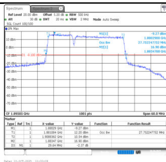
2-2-10MHz-20MHz-16QAM-16QAM-18956-19100-50RB#0-100RB#0-PASS
