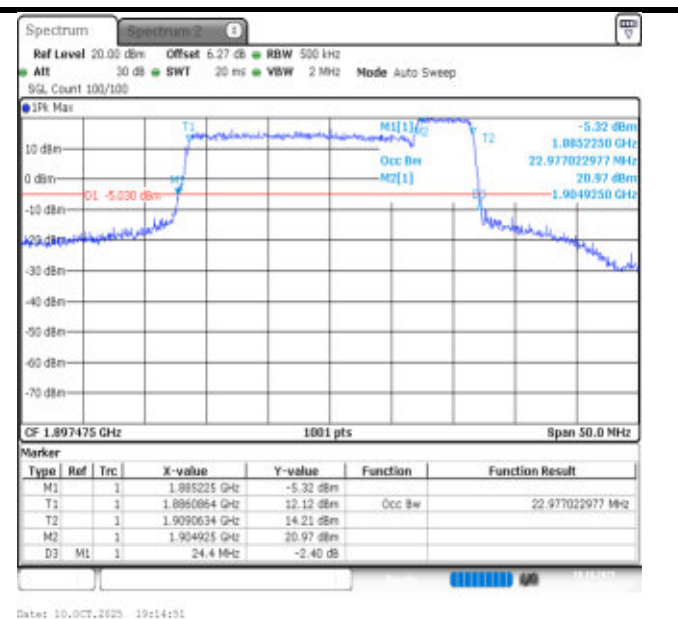
2-2-20MHz-5MHz-16QAM-16QAM-19050-19167-100RB#0-25RB#0-PASS
