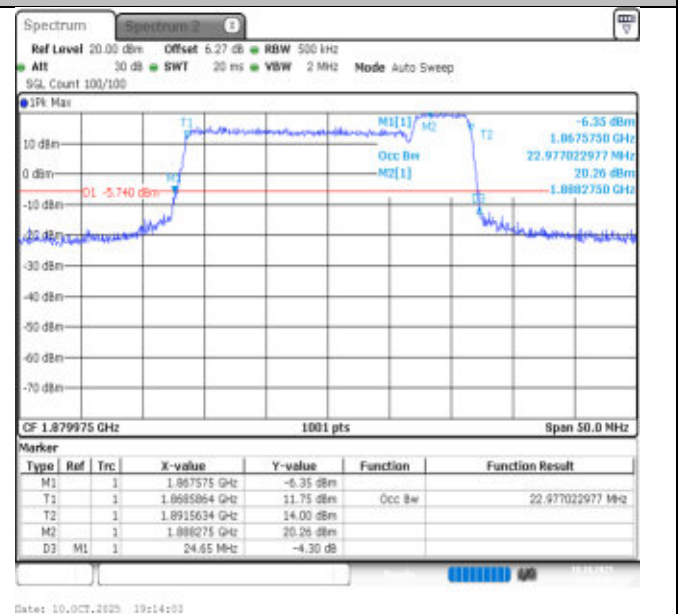
2-2-20MHz-5MHz-16QAM-16QAM-18875-18992-100RB#0-25RB#0-PASS
