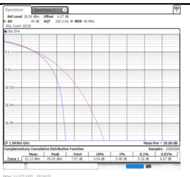
2-2-20MHz-15MHz-16QAM-16QAM-18951-19122-100RB#0-75RB#0-PASS
