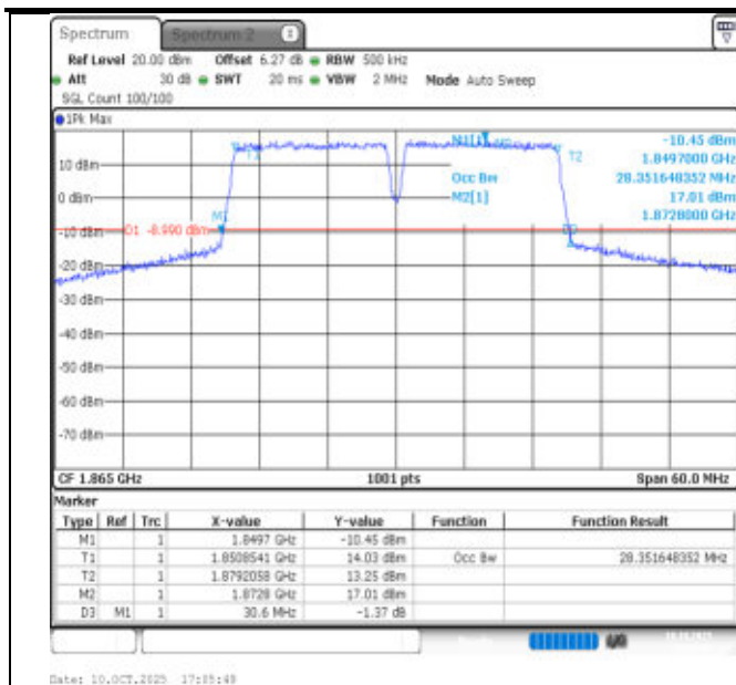
2-2-15MHz-15MHz-QPSK-QPSK-18675-18825-75RB#0-75RB#0-PASS
