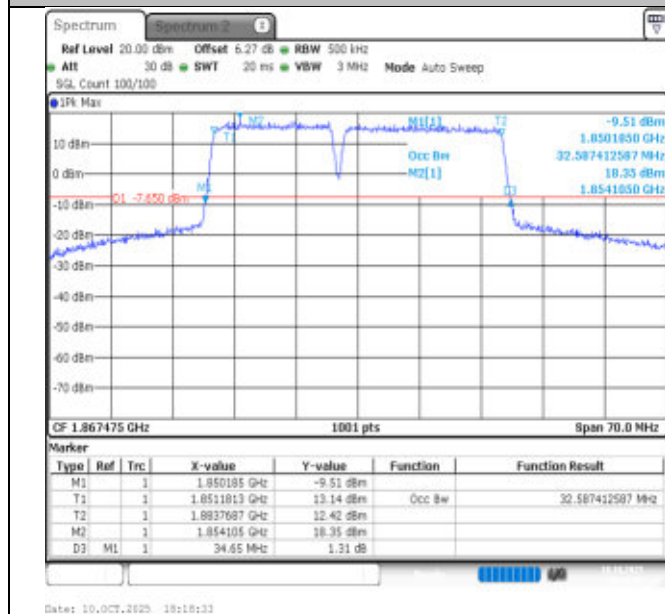
2-2-15MHz-20MHz-QPSK-QPSK-18678-18849-75RB#0-100RB#0-PASS
