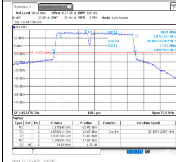
2-2-15MHz-20MHz-QPSK-QPSK-18929-19100-75RB#0-100RB#0-PASS
