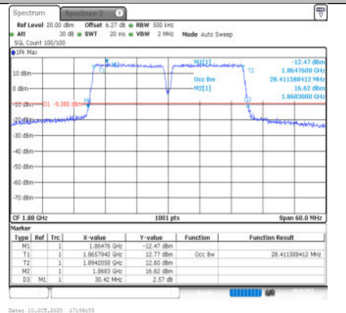
2-2-15MHz-15MHz-16QAM-16QAM-18825-18975-75RB#0-75RB#0-PASS
