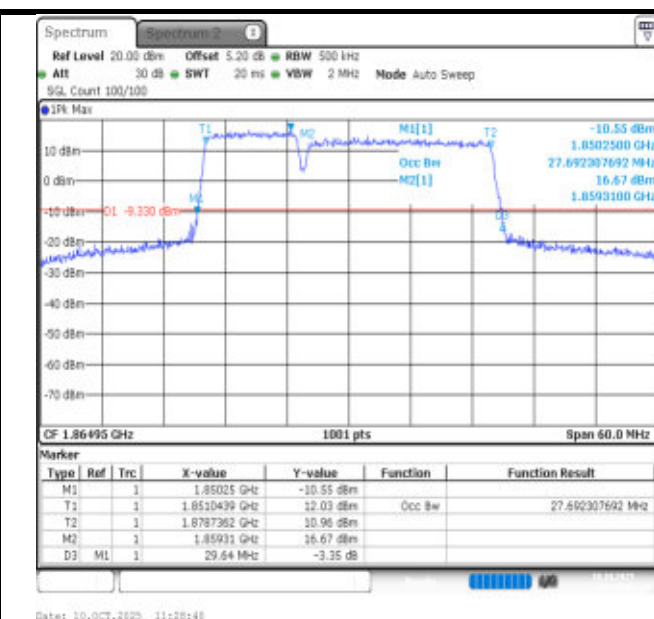
2-2-10MHz-20MHz-16QAM-16QAM-18655-18799-50RB#0-100RB#0-PASS
