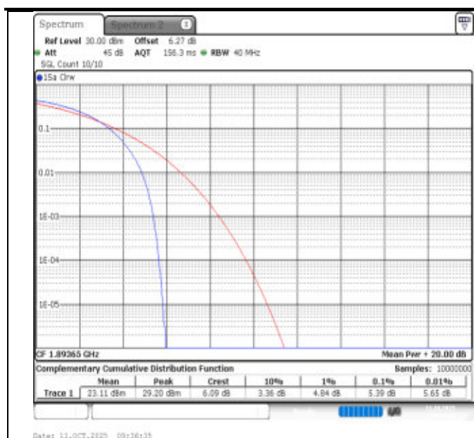
2-2-20MHz-15MHz-QPSK-QPSK-18951-19122-100RB#0-75RB#0-PASS
