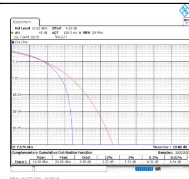
41-41-15MHz-15MHz-16QAM-16QAM-41365-41515-75RB#0-75RB#0-PASS
