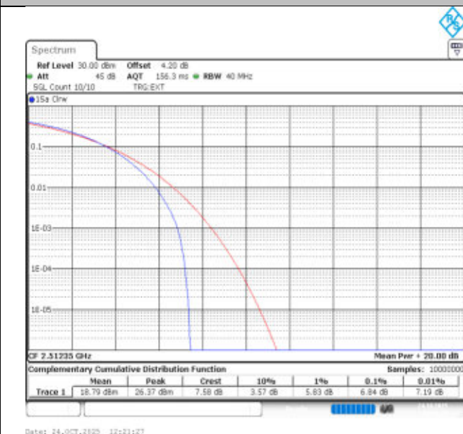
41-41-15MHz-20MHz-16QAM-16QAM-39728-39899-75RB#0-100RB#0-PASS
