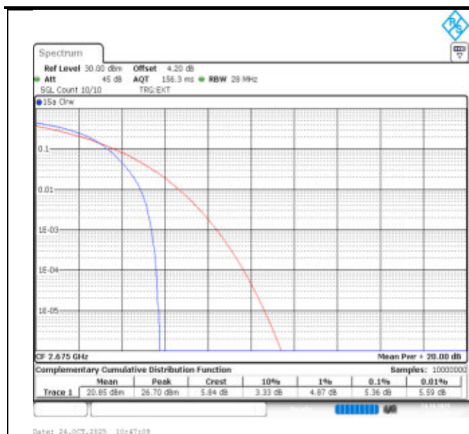
41-41-15MHz-15MHz-QPSK-QPSK-41365-41515-75RB#0-75RB#0-PASS
