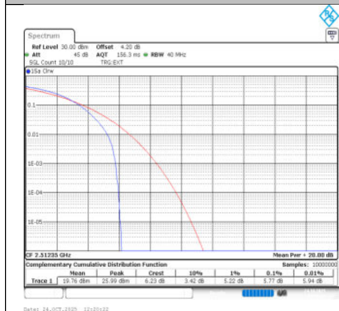
41-41-15MHz-20MHz-QPSK-QPSK-39728-39899-75RB#0-100RB#0-PASS
