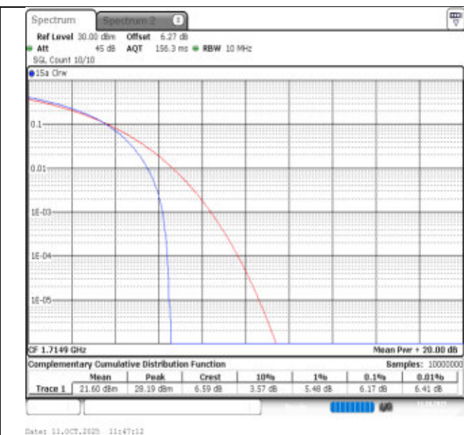
66-66-5MHz-5MHz-16QAM-16QAM-131997-132045-25RB#0-25RB#0-PASS
