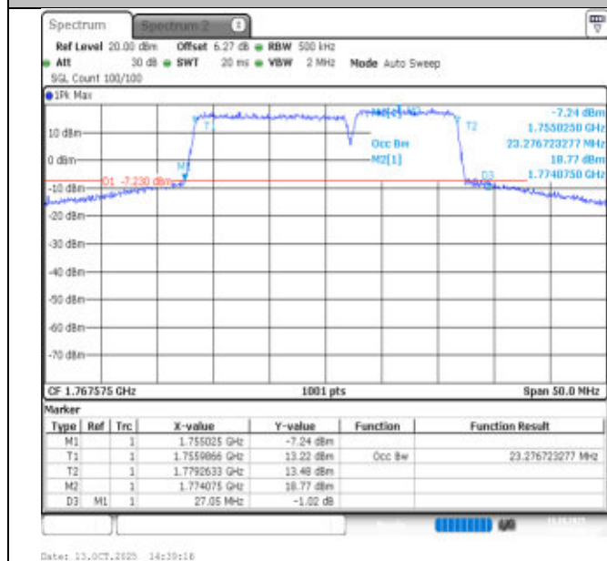
66-66-15MHz-10MHz-QPSK-QPSK-132499-132619-75RB#0-50RB#0-PASS
