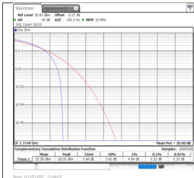
66-66-5MHz-5MHz-QPSK-QPSK-131997-132045-25RB#0-25RB#0-PASS
