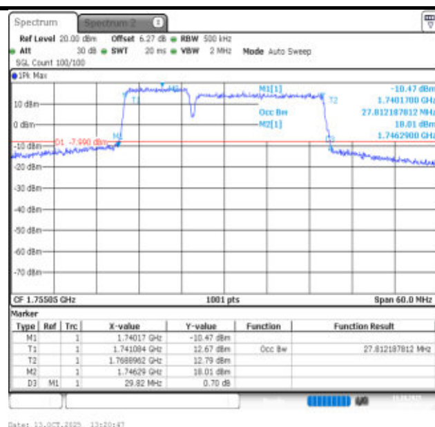
66-66-10MHz-20MHz-16QAM-16QAM-132328-132472-50RB#0-100RB#0-PASS
