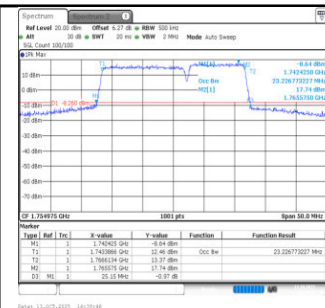
66-66-15MHz-10MHz-16QAM-16QAM-132373-132493-75RB#0-50RB#0-PASS
