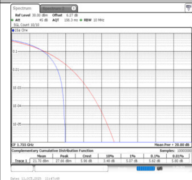
66-66-5MHz-5MHz-16QAM-16QAM-132398-132446-25RB#0-25RB#0-PASS
