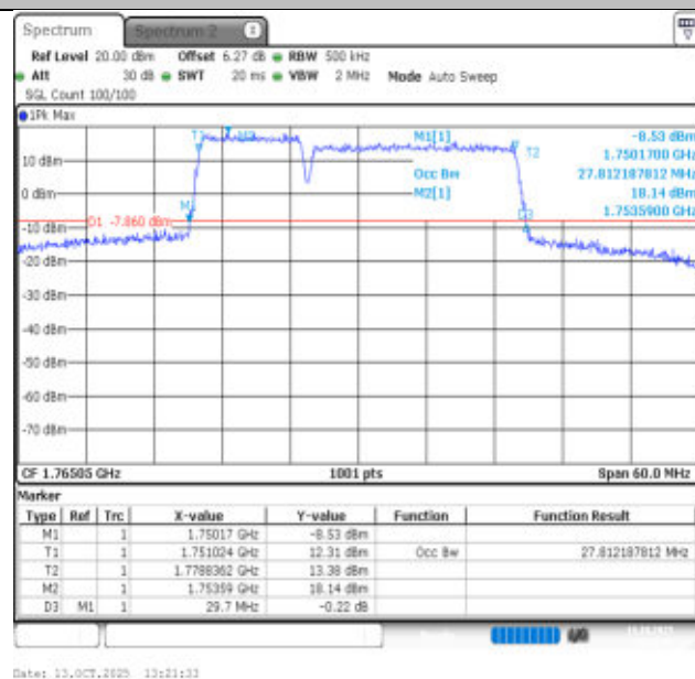
66-66-10MHz-20MHz-16QAM-16QAM-132428-132572-50RB#0-100RB#0-PASS
