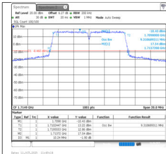
66-66-5MHz-5MHz-QPSK-QPSK-131997-132045-25RB#0-25RB#0-PASS
