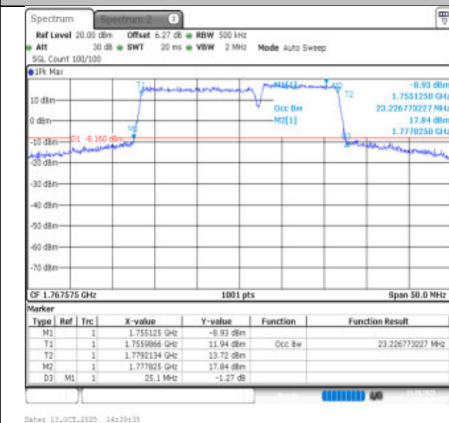
66-66-15MHz-10MHz-16QAM-16QAM-132499-132619-75RB#0-50RB#0-PASS
